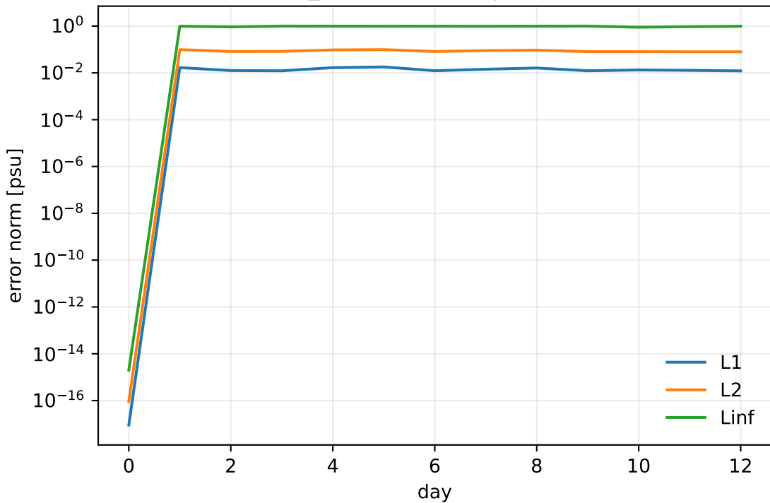
advect_cs error norms | alpha=0.05
