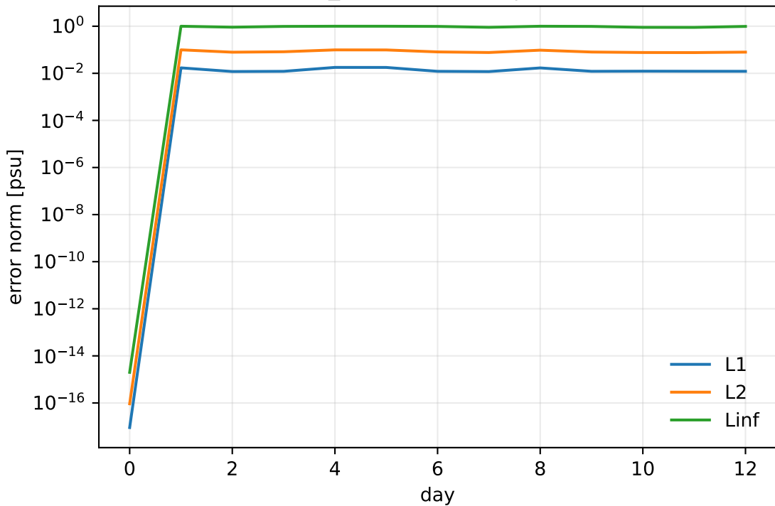
advect_cs error norms | alpha=0
