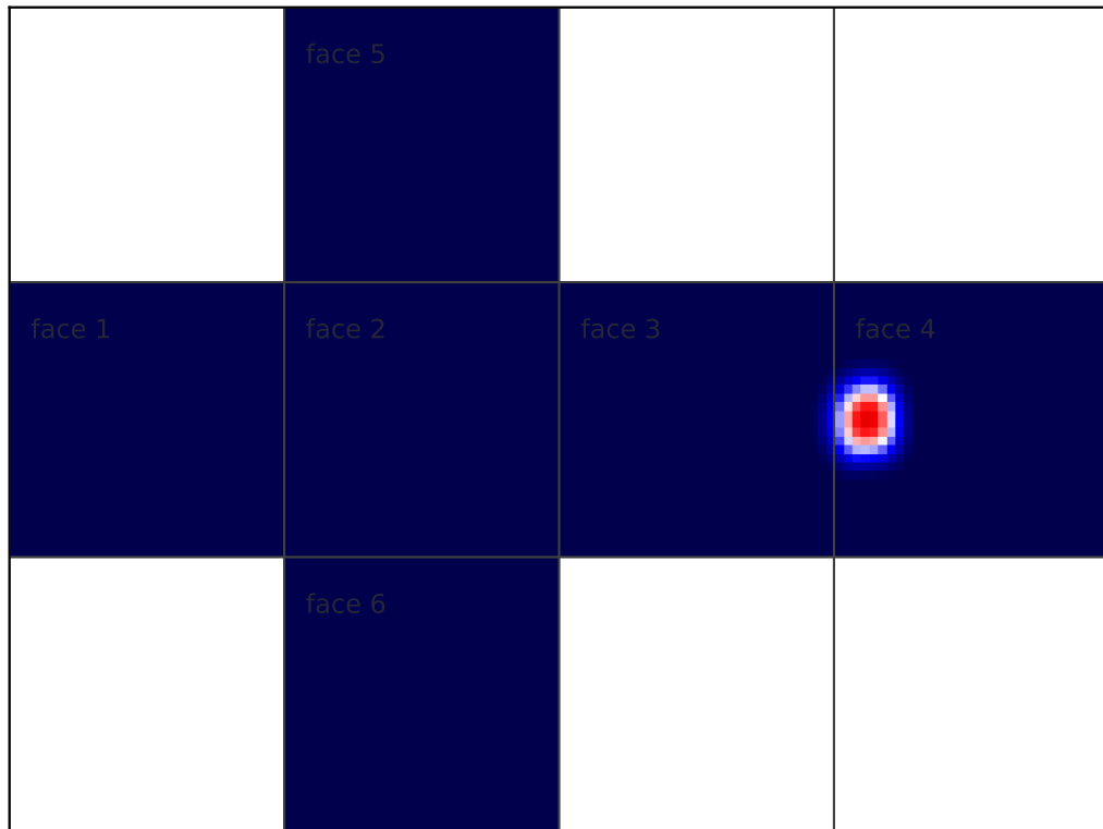
advect_cs final model tracer | alpha=0
