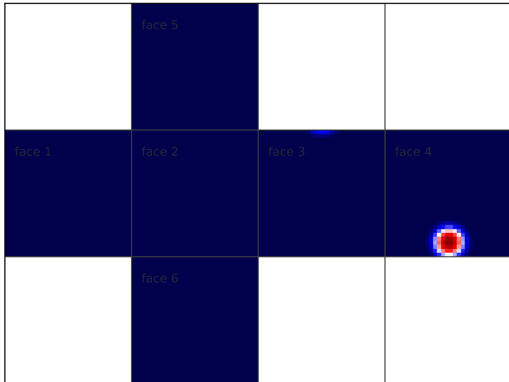
advect_cs final exact tracer | alpha=1.52
