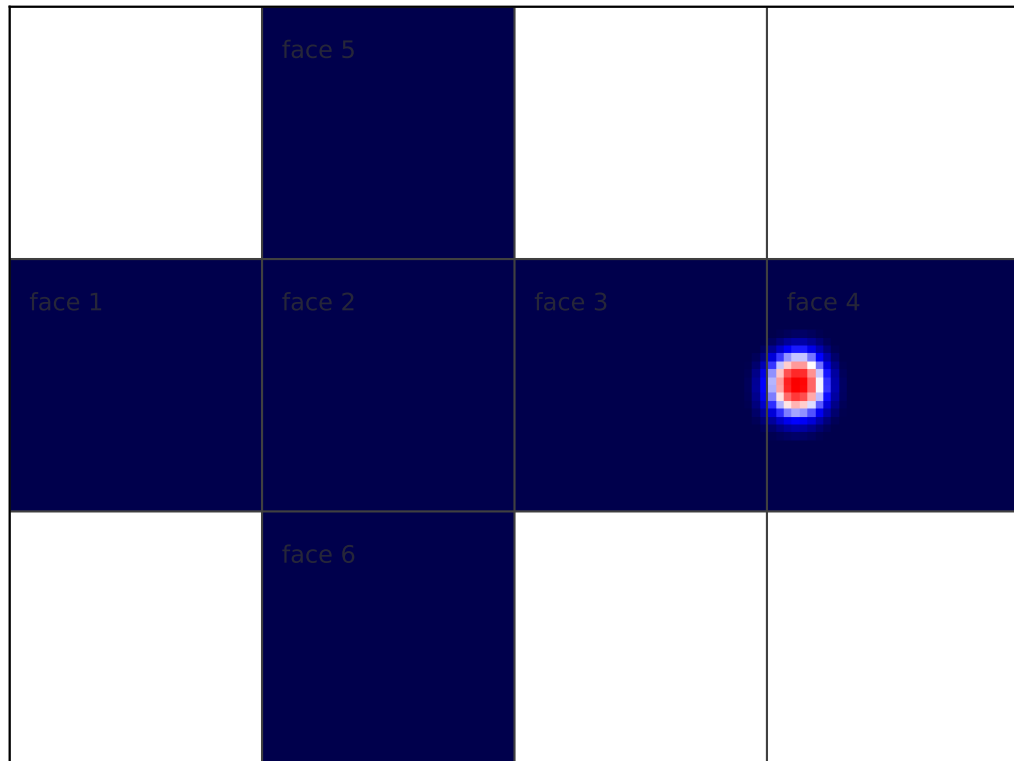
advect_cs final model tracer | \alpha=1.52
