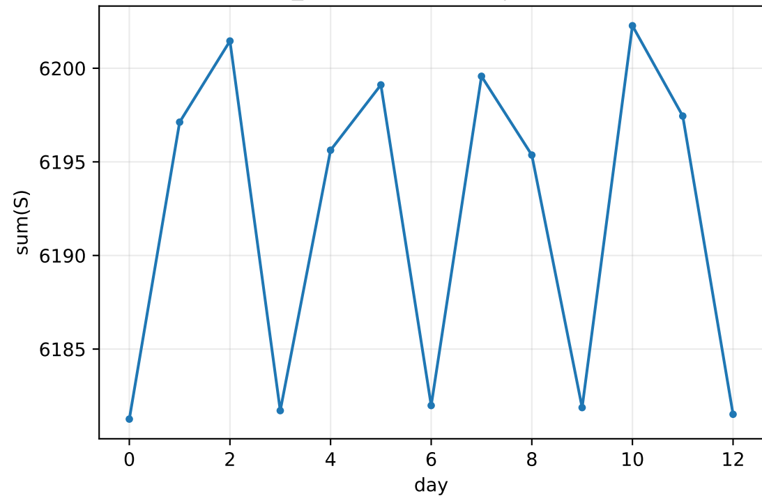
advect_cs tracer integral | alpha=0.05
