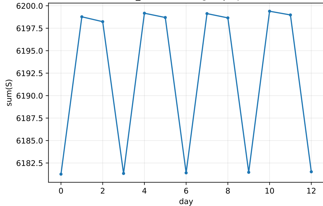
advect_cs tracer integral | alpha=0
