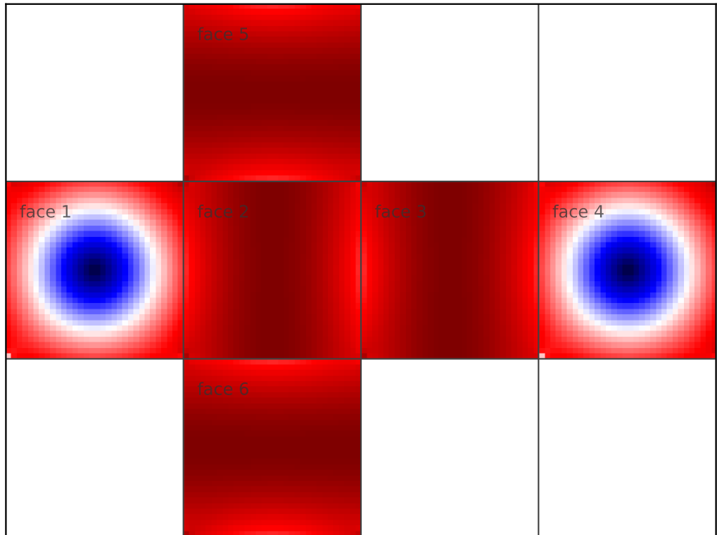
advect_cs velocity magnitude | alpha=1.57
