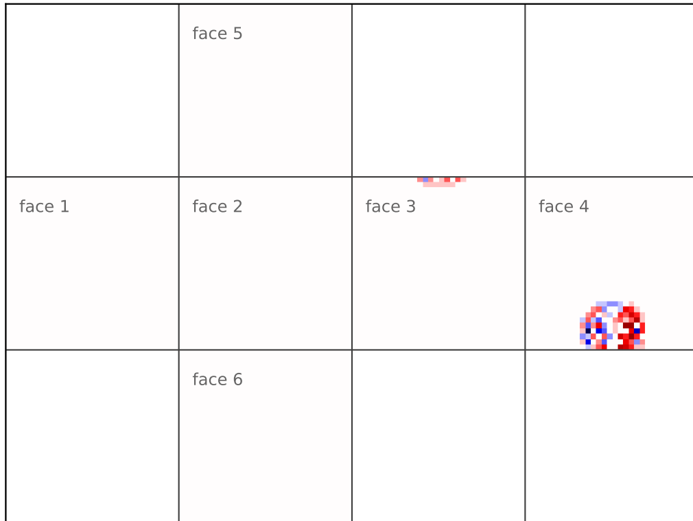
advect_cs S error | alpha=0 | day=0.00
