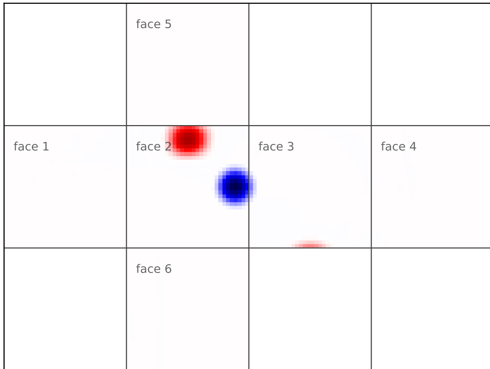
advect_cs S error | alpha=0 | day=9.00
