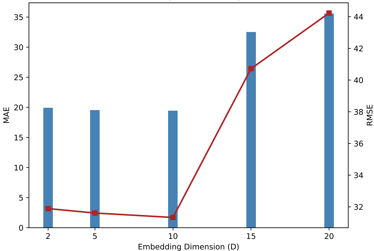
PEMS04: Sensitivity to Embedding Dimension
