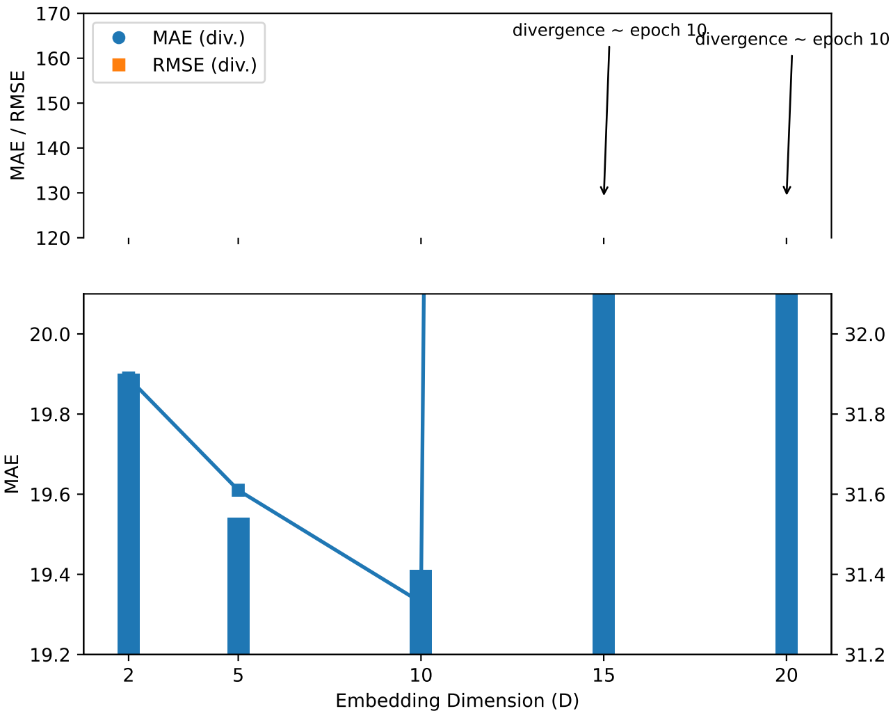
PEMS04: Sensitivity to Embedding Dimension (Broken Axis for Divergence)
