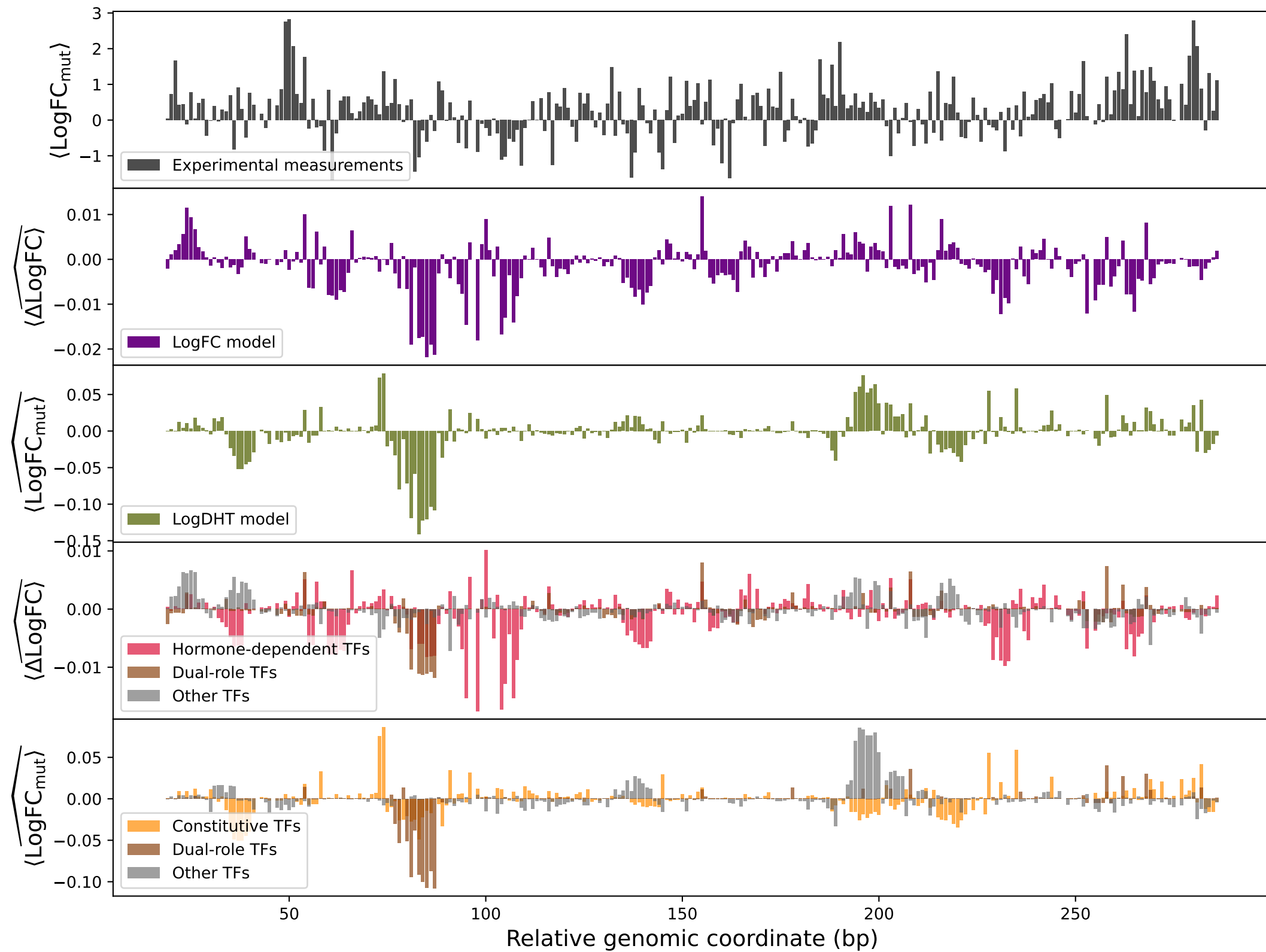
peakno_528
