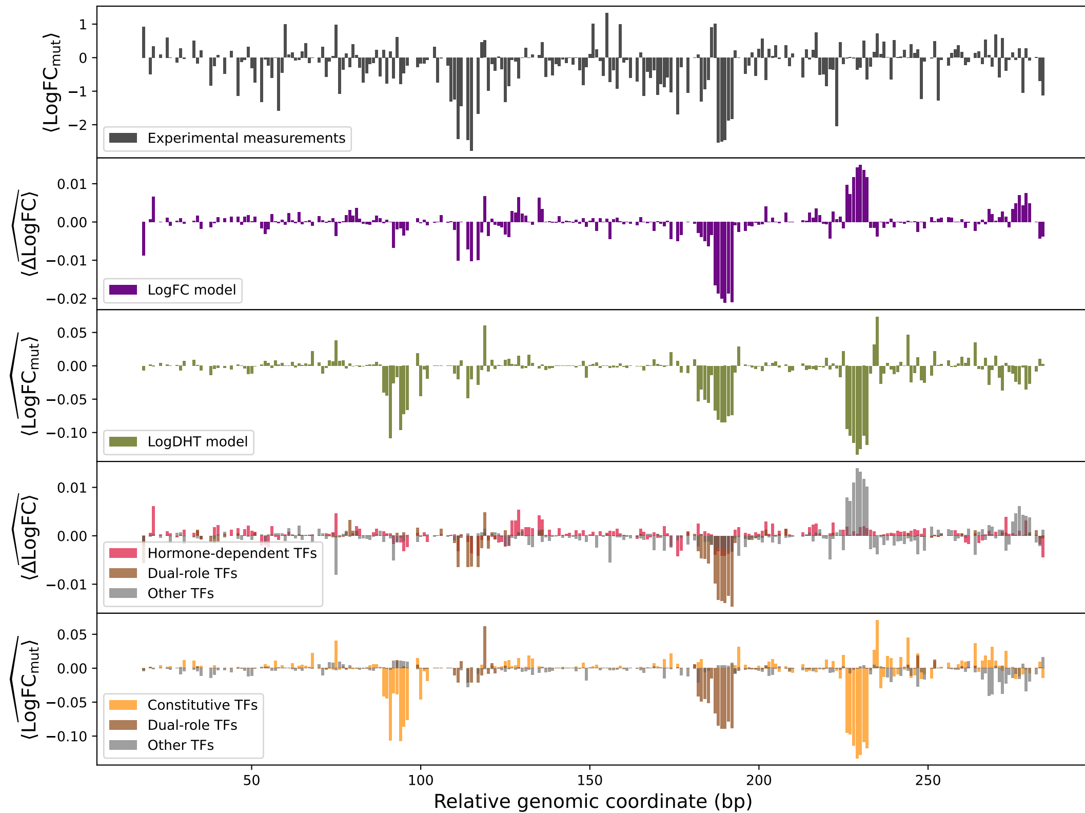
peakno_1021
