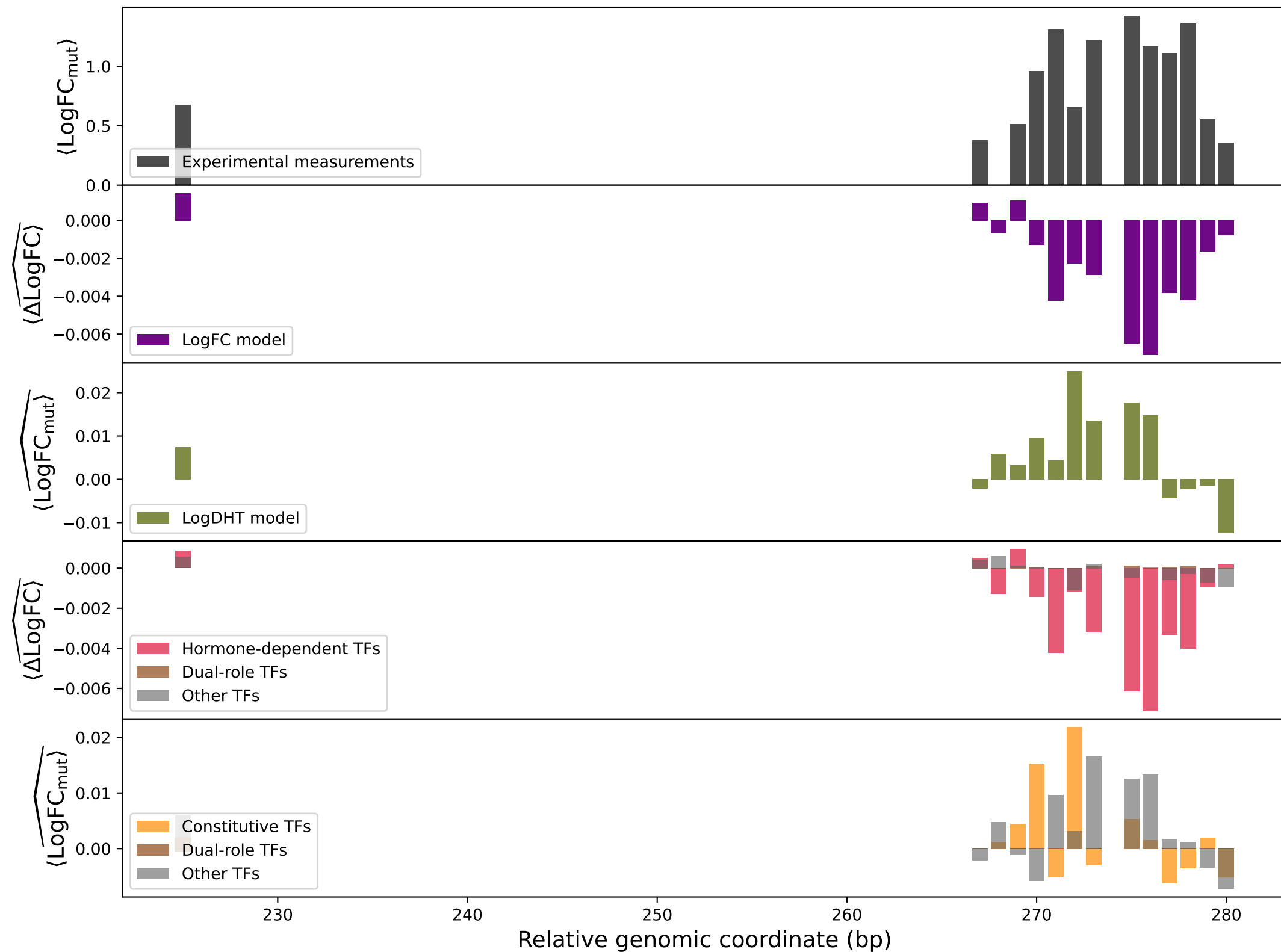
peakno_2221
