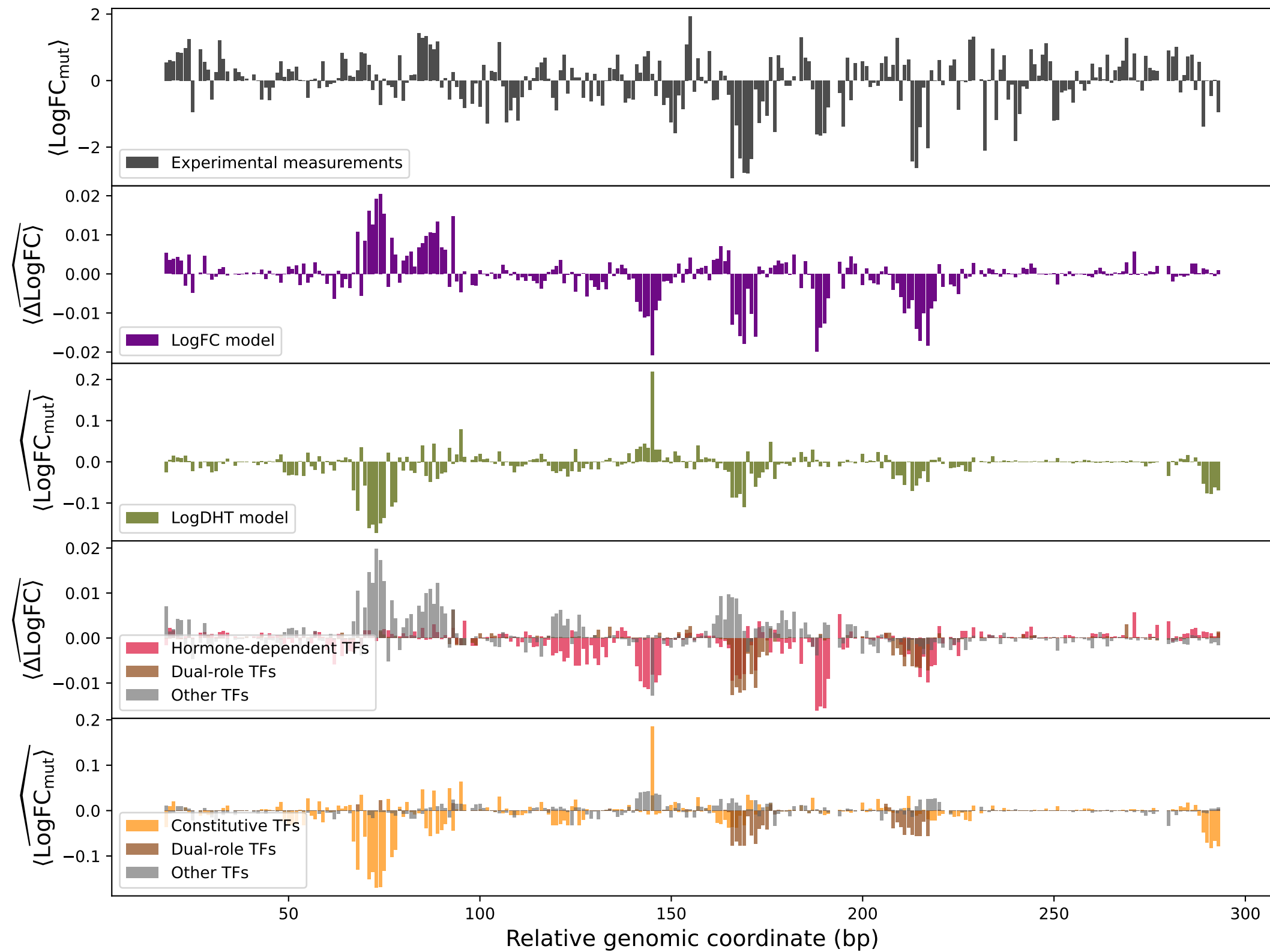
peakno_2261
