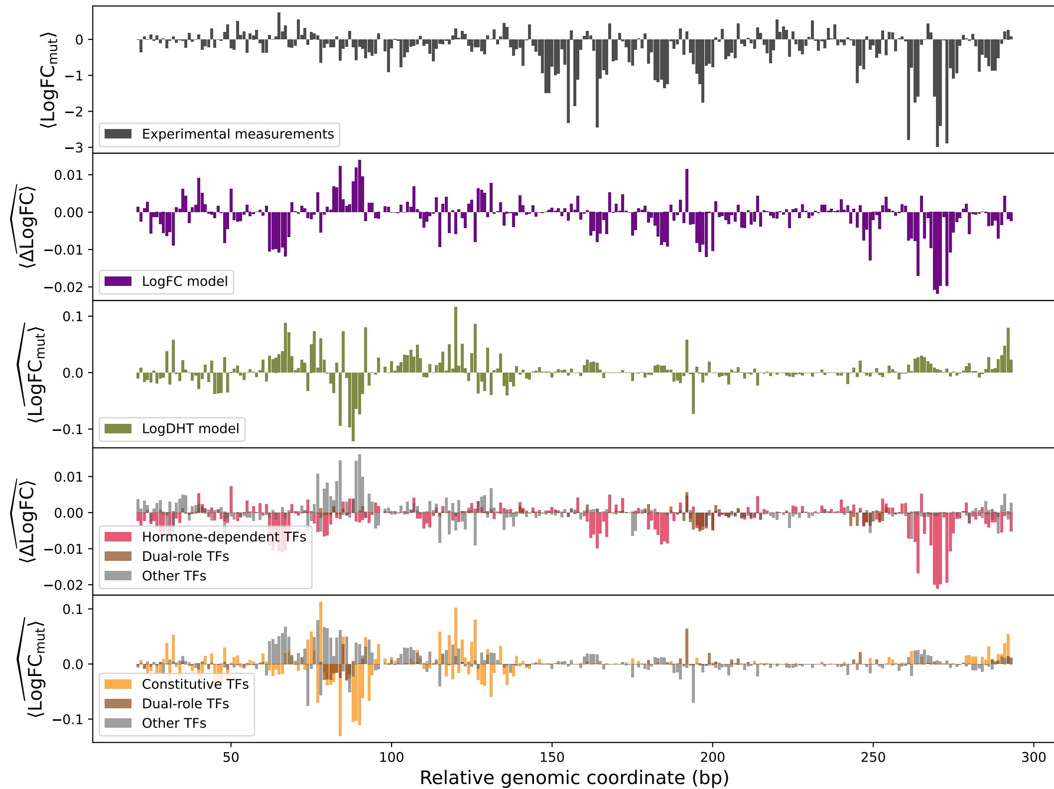
peakno_2022
