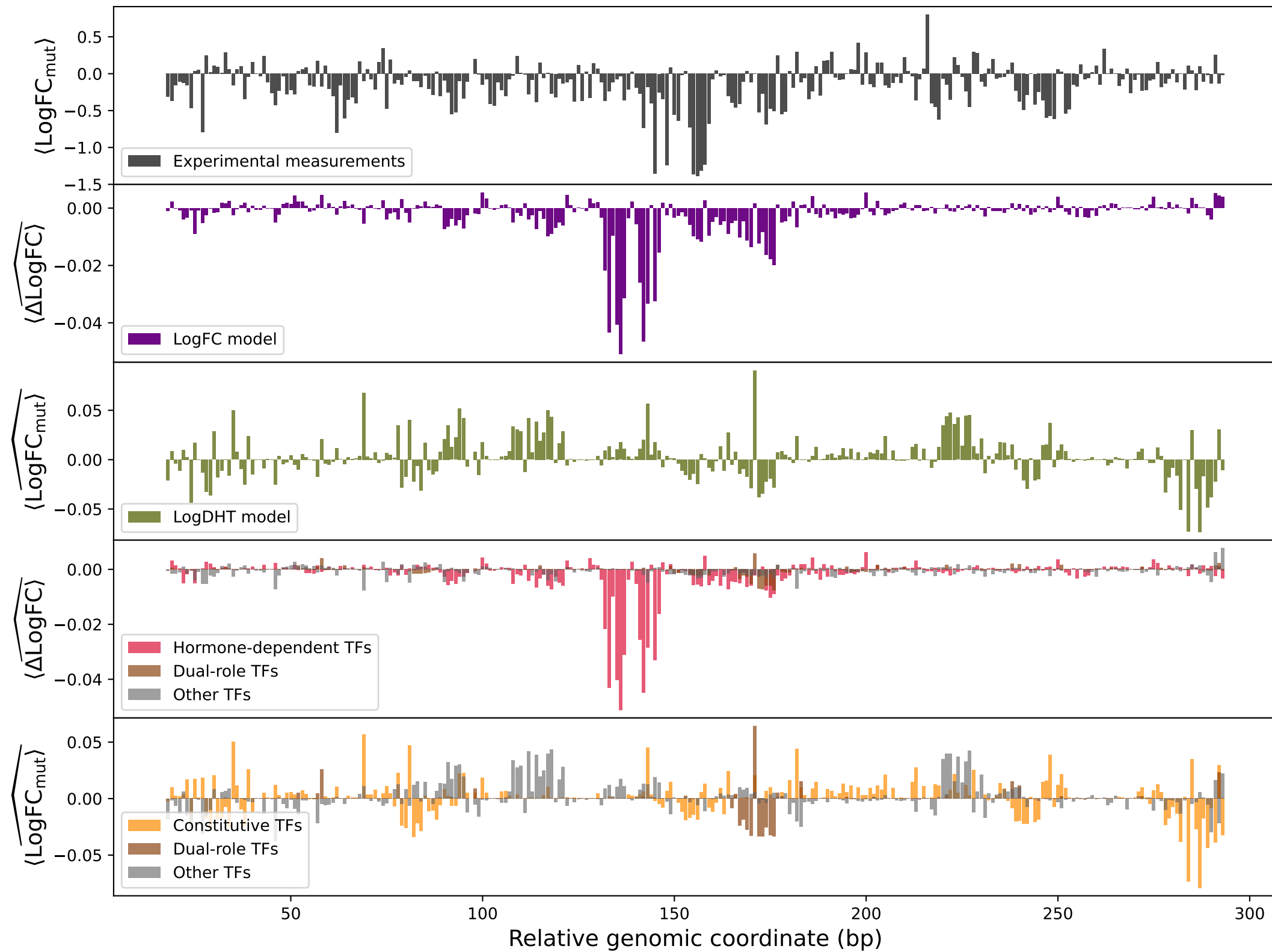
overlapped_read_612
