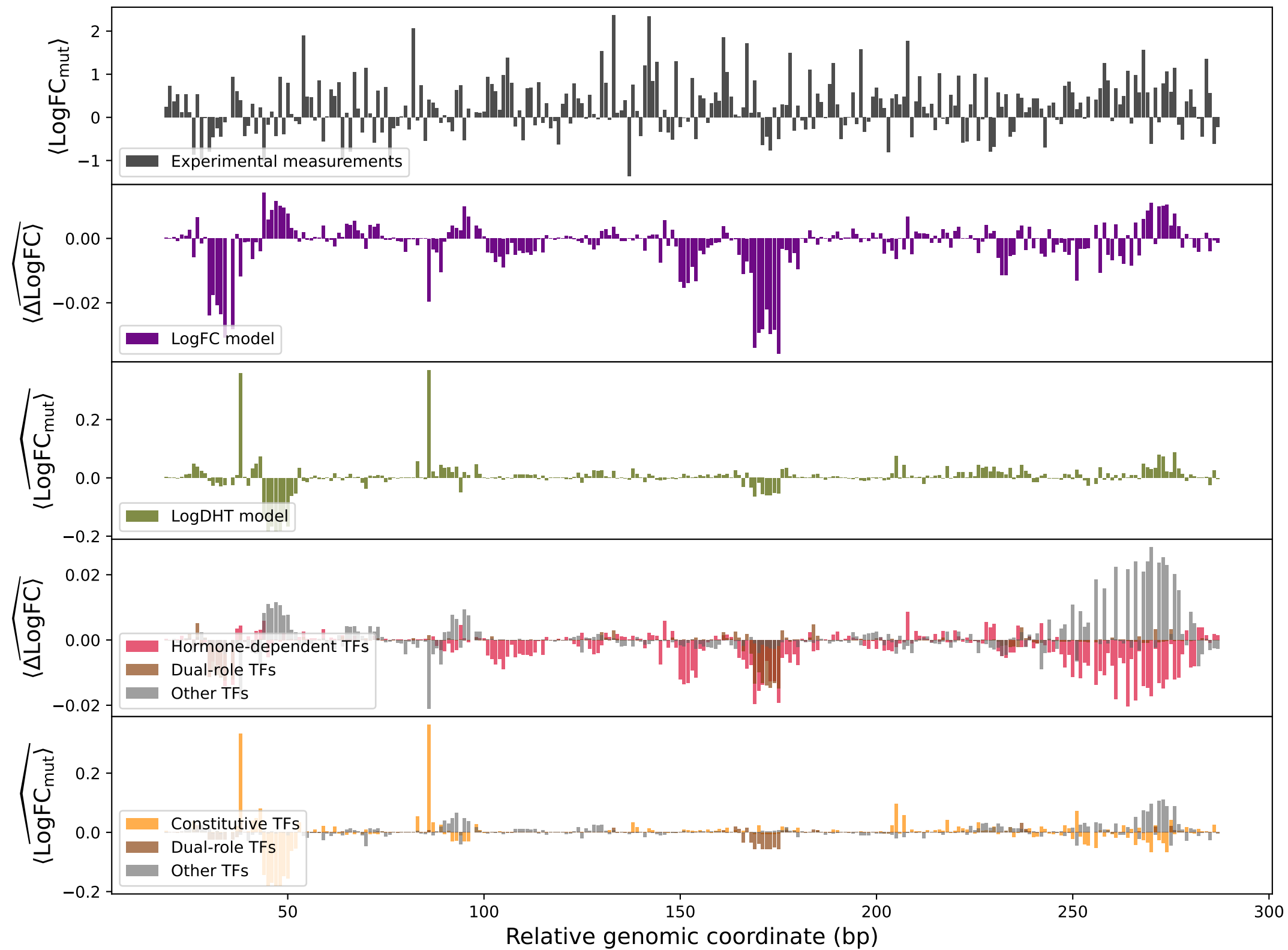
peakno_2862
