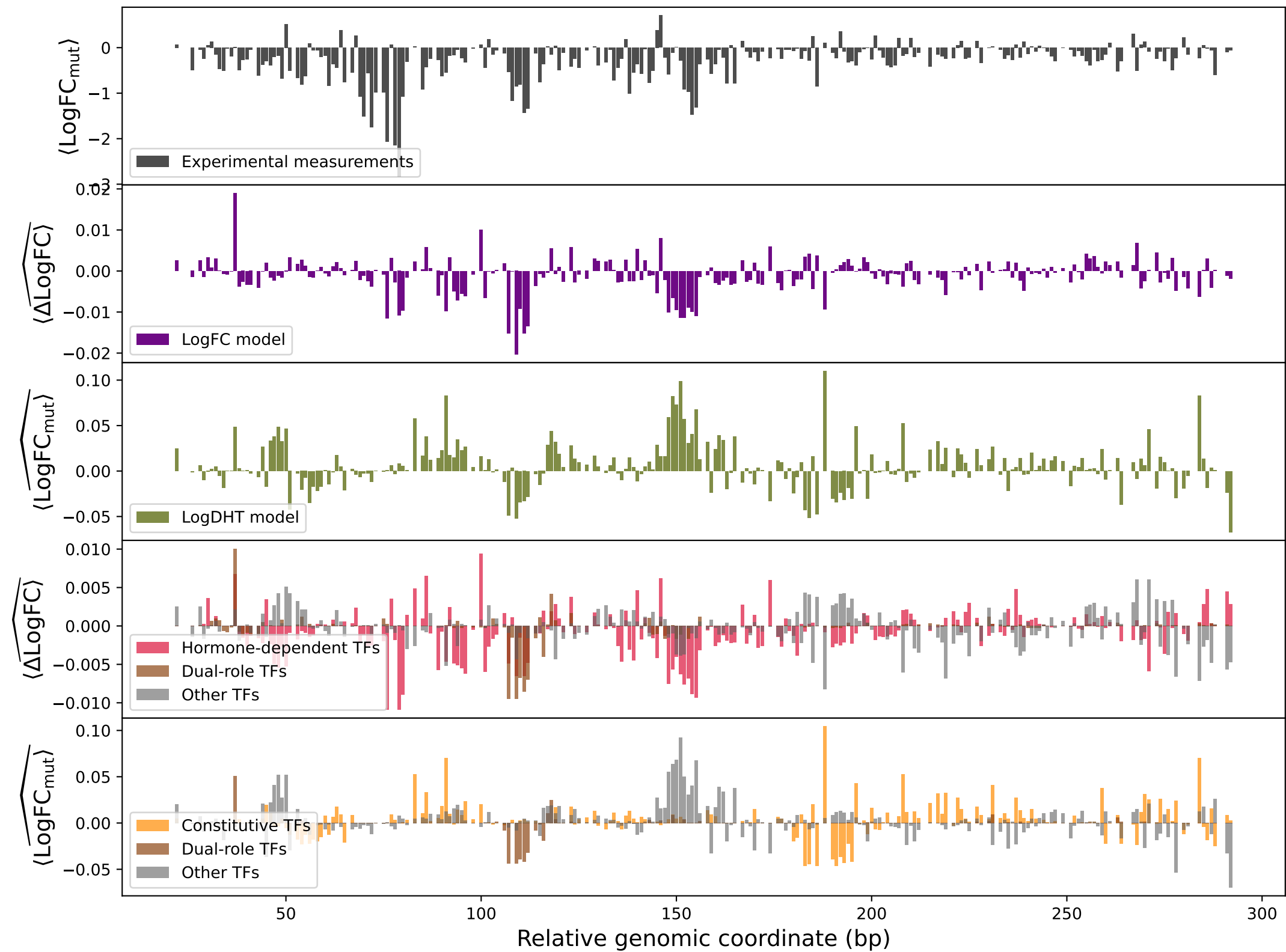
overlapped_read_56
