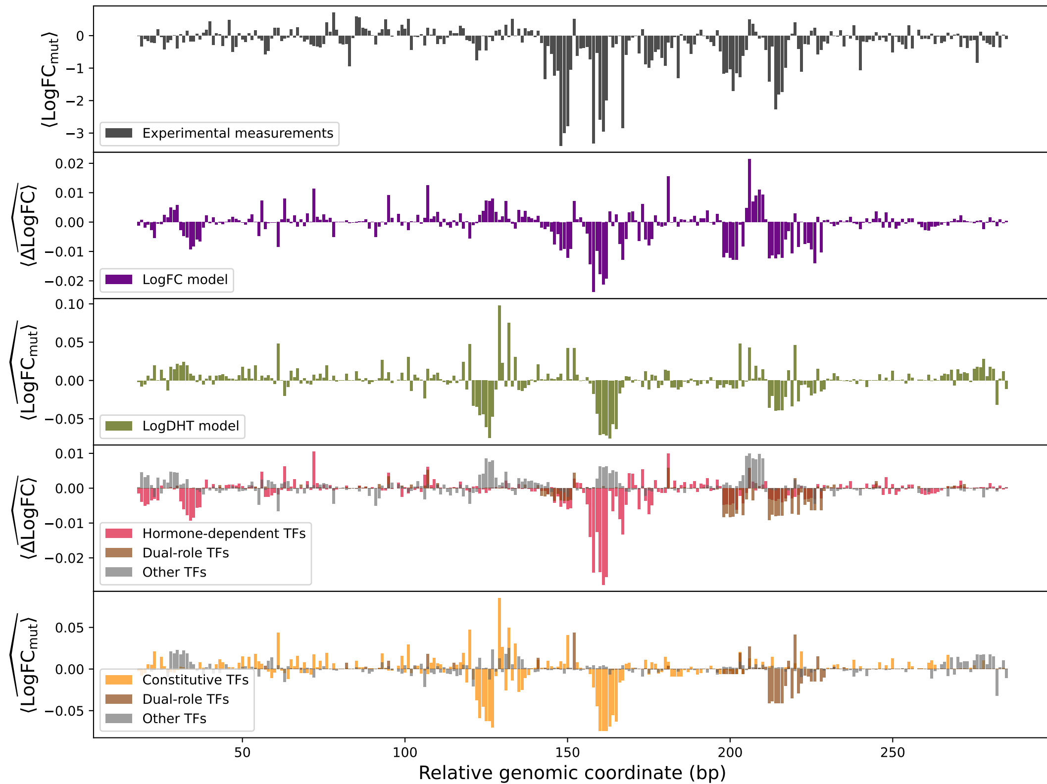
peakno_675
