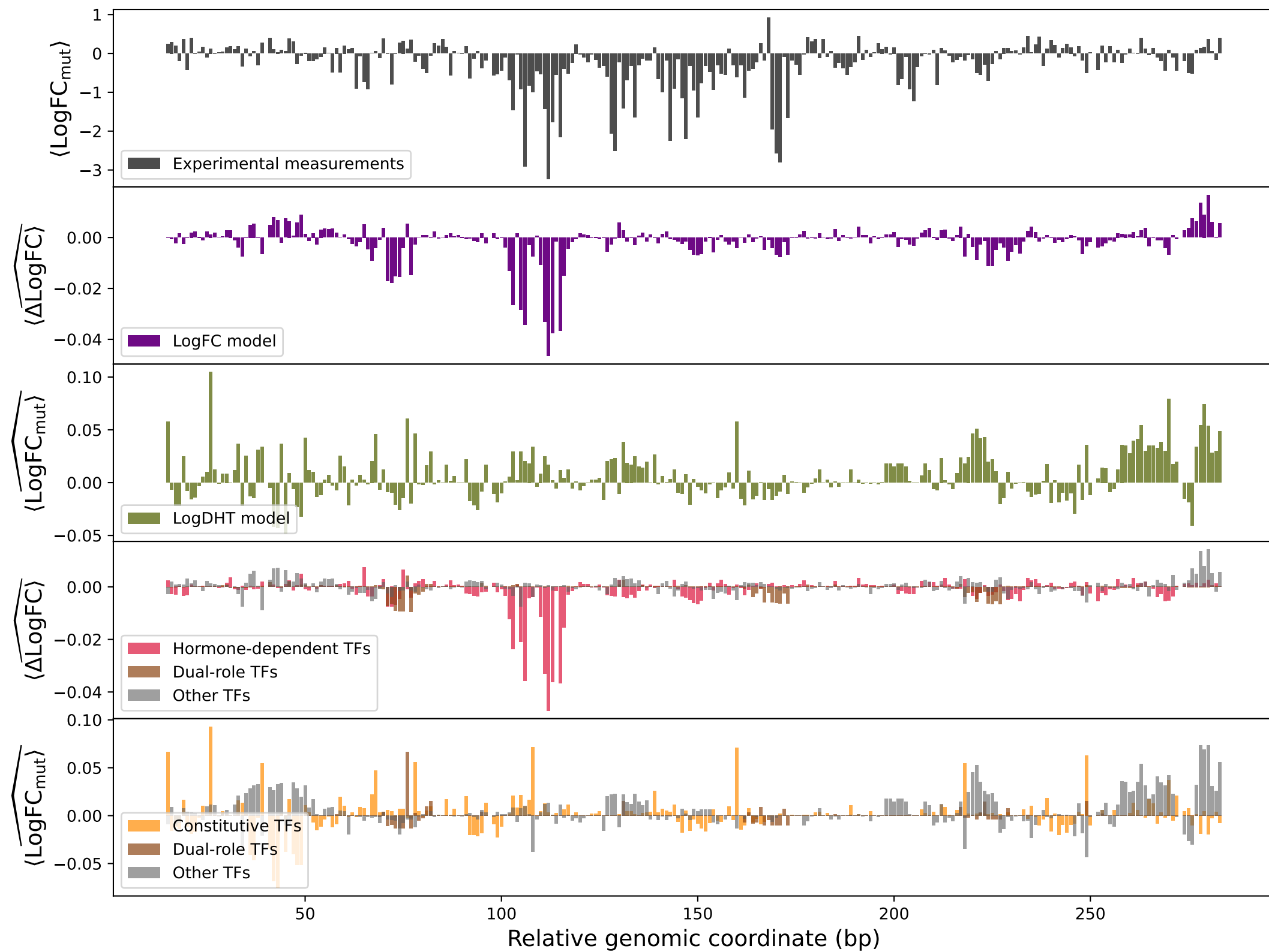
overlapped_read_659
