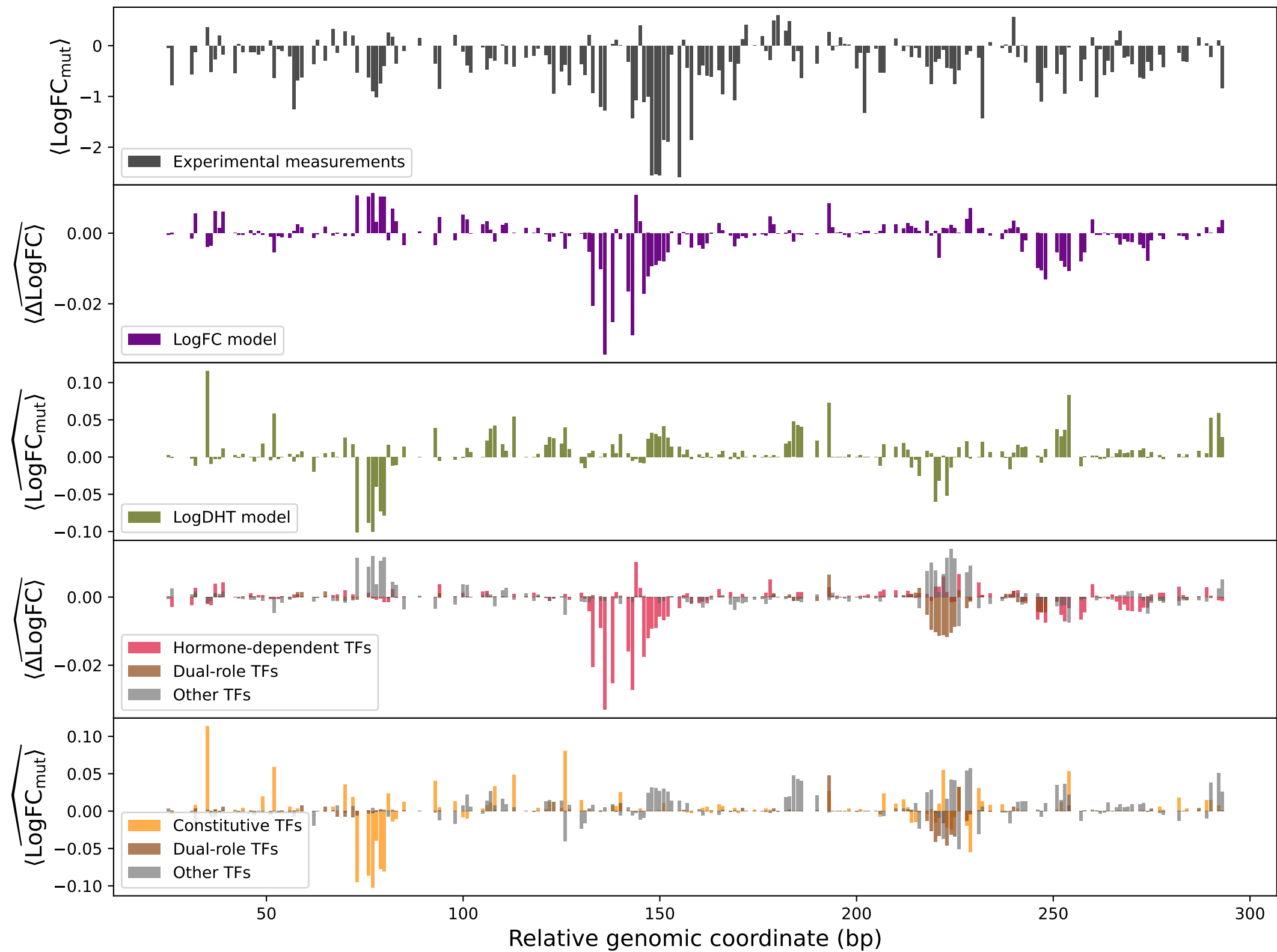
peakno_789
