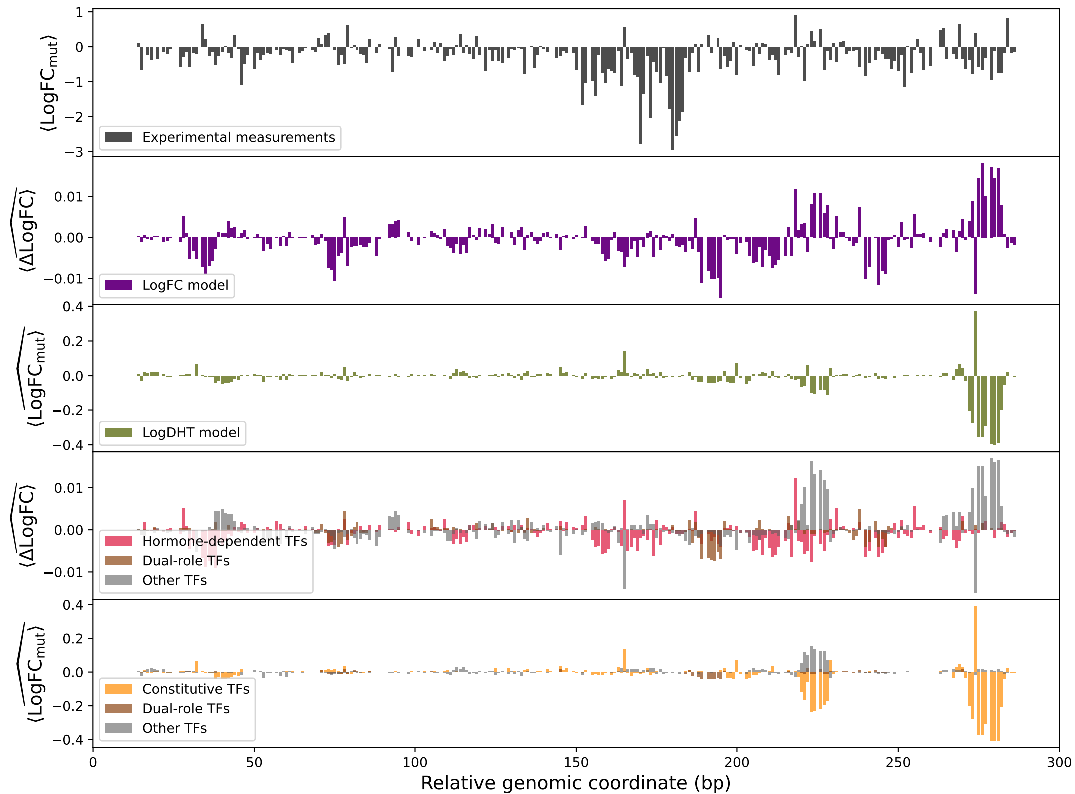
overlapped_read_114
