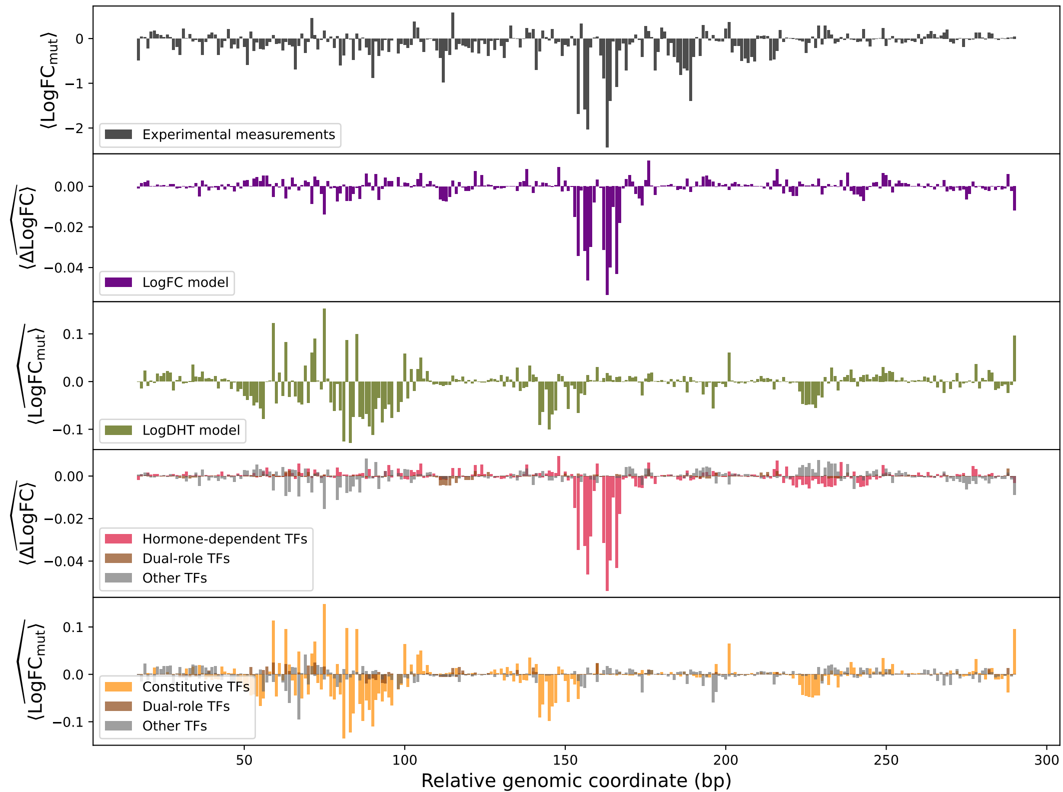
overlapped_read_509
