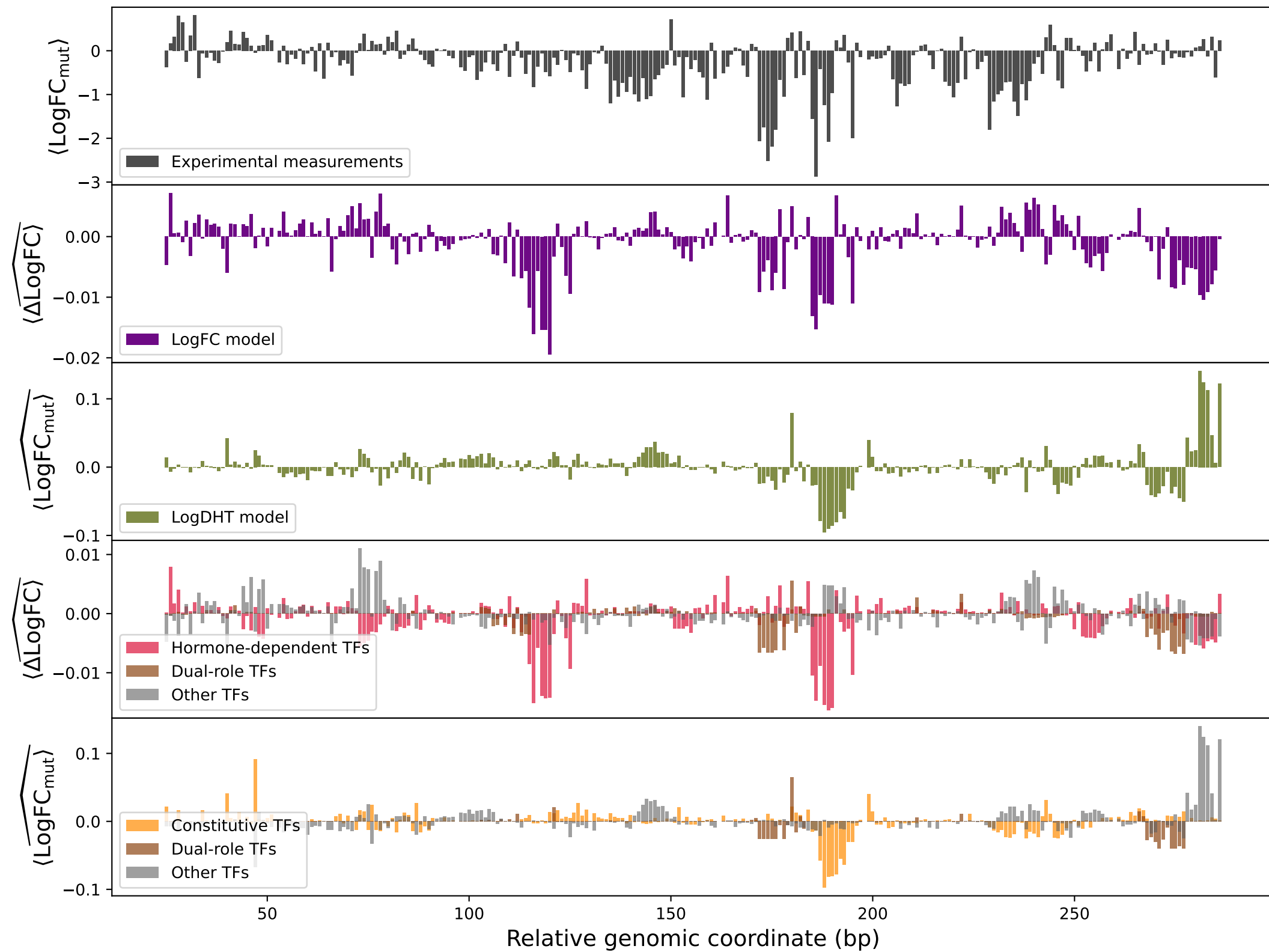
peakno_332
