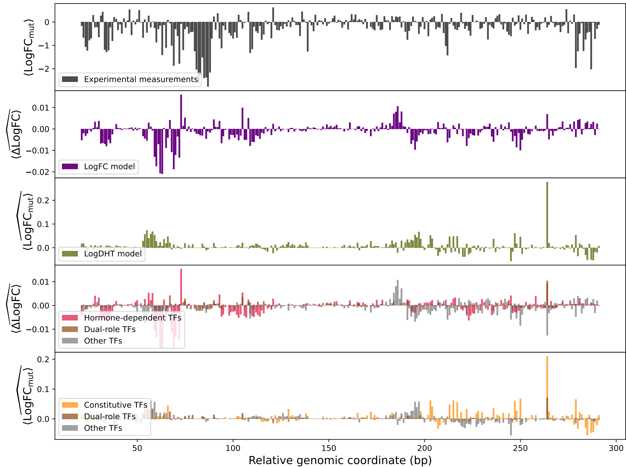
peakno_2415
