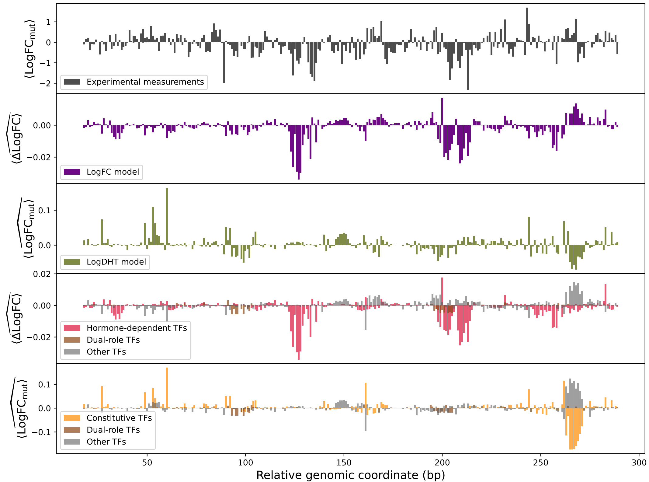
peakno_415
