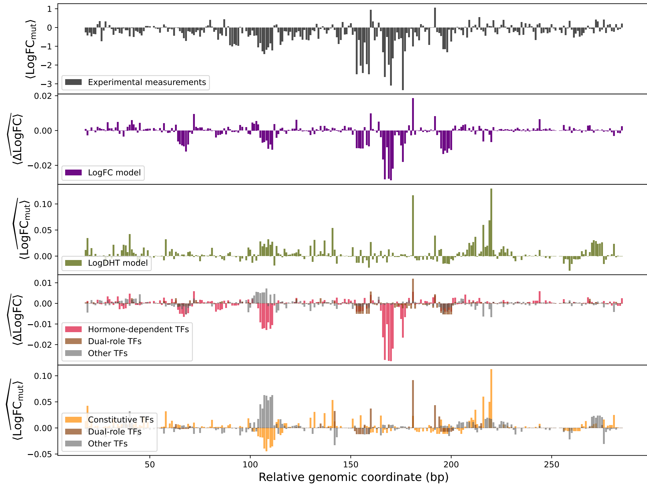
peakno_143
