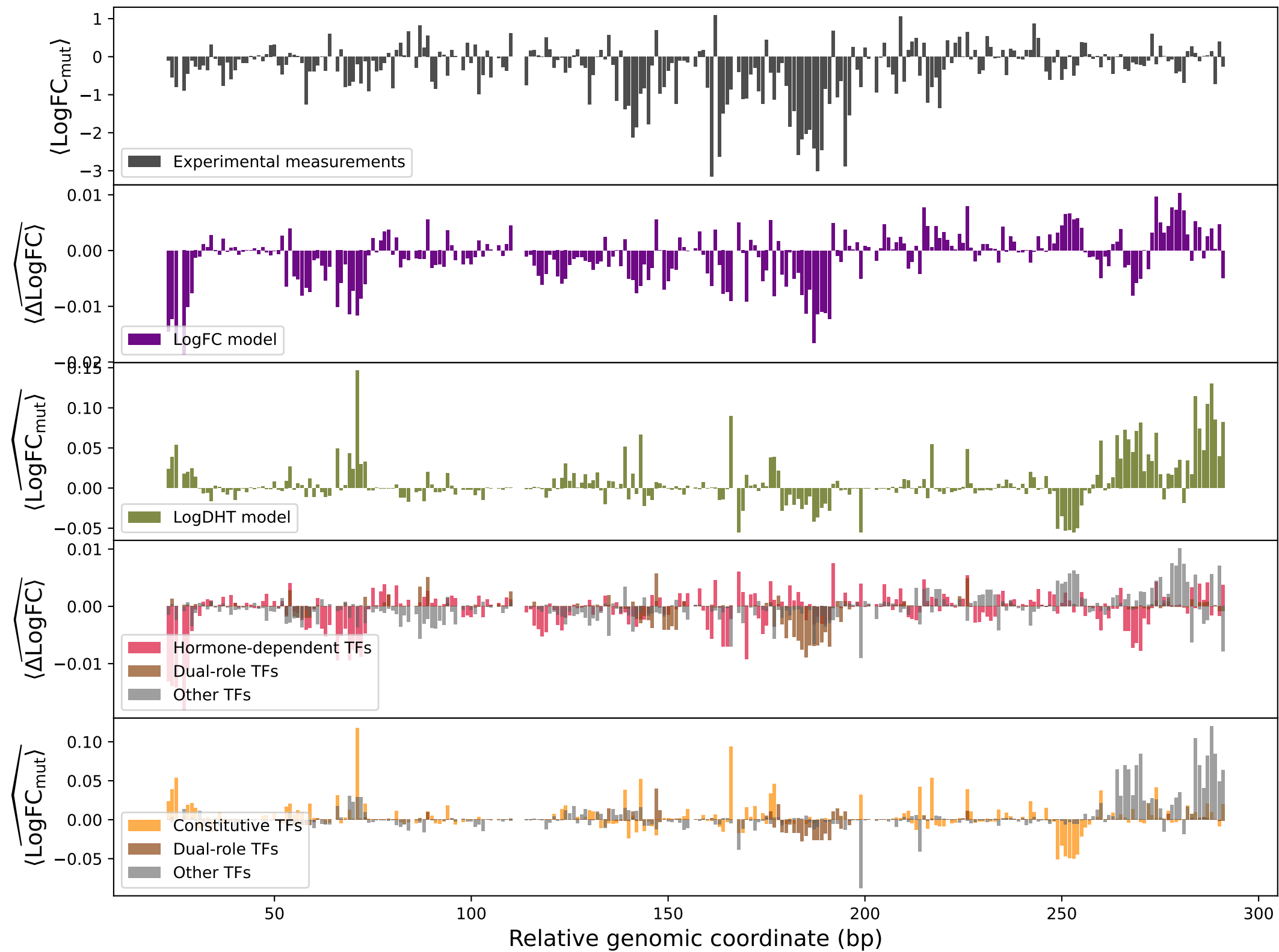
peakno_768
