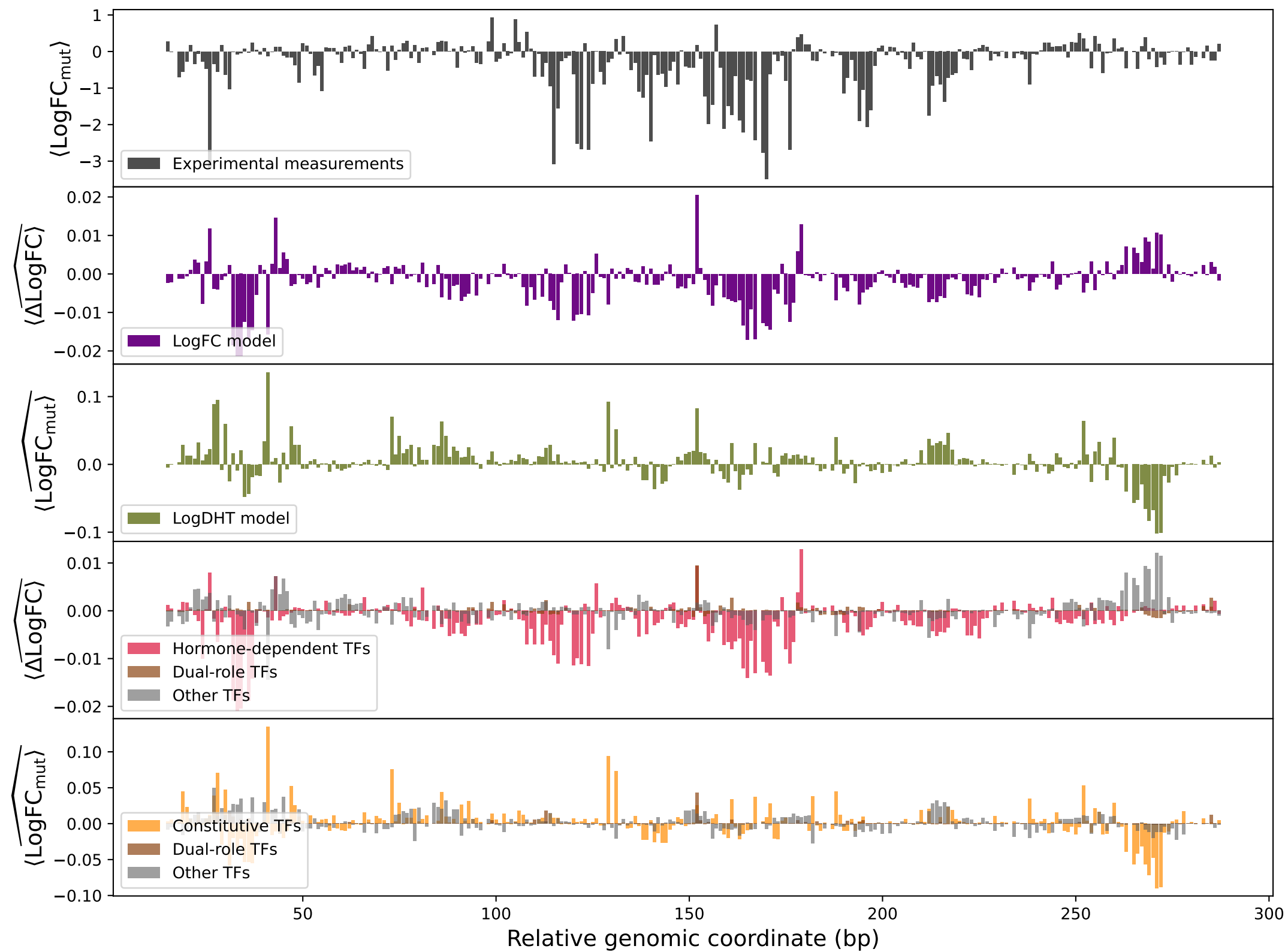
overlapped_read_167
