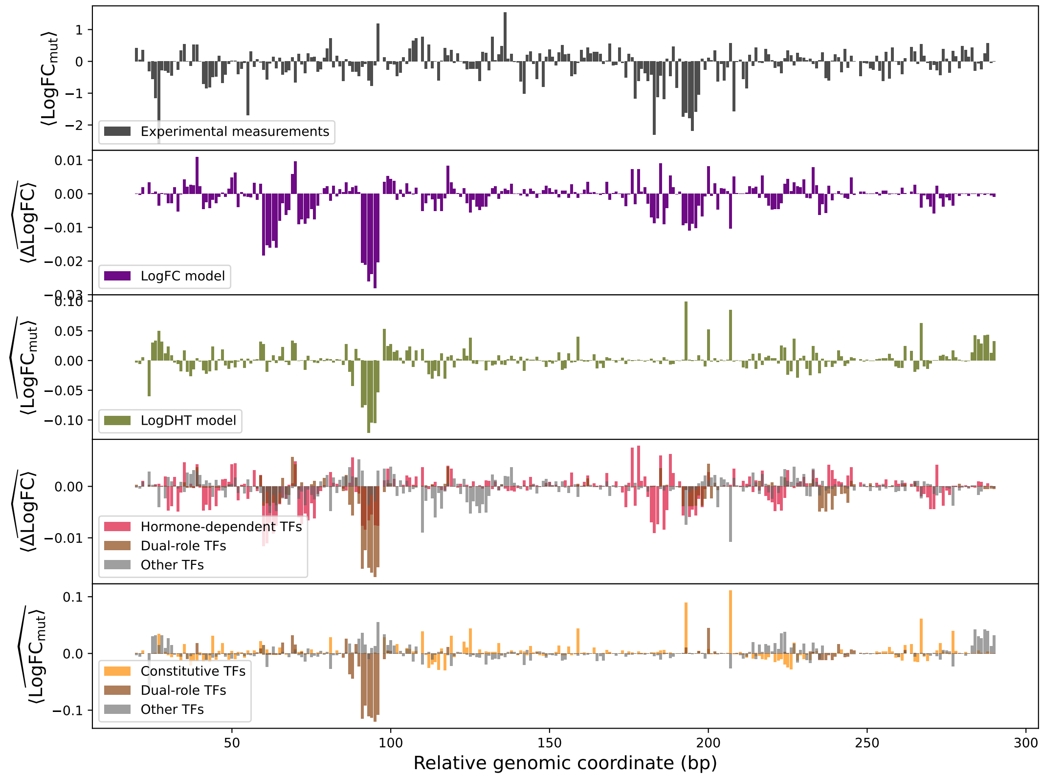
peakno_799
