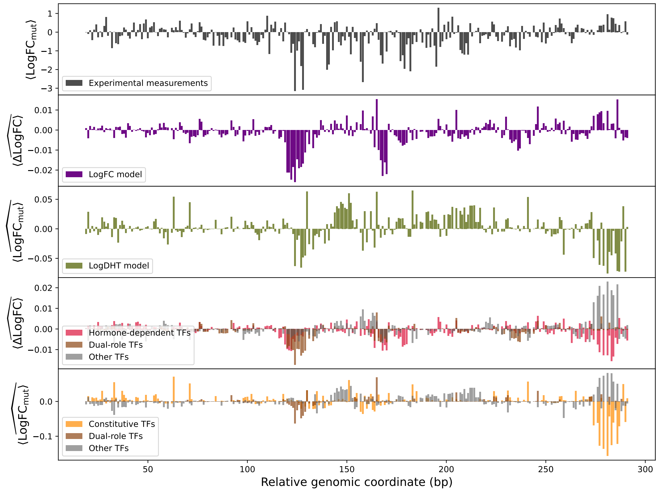
overlapped_read_73
