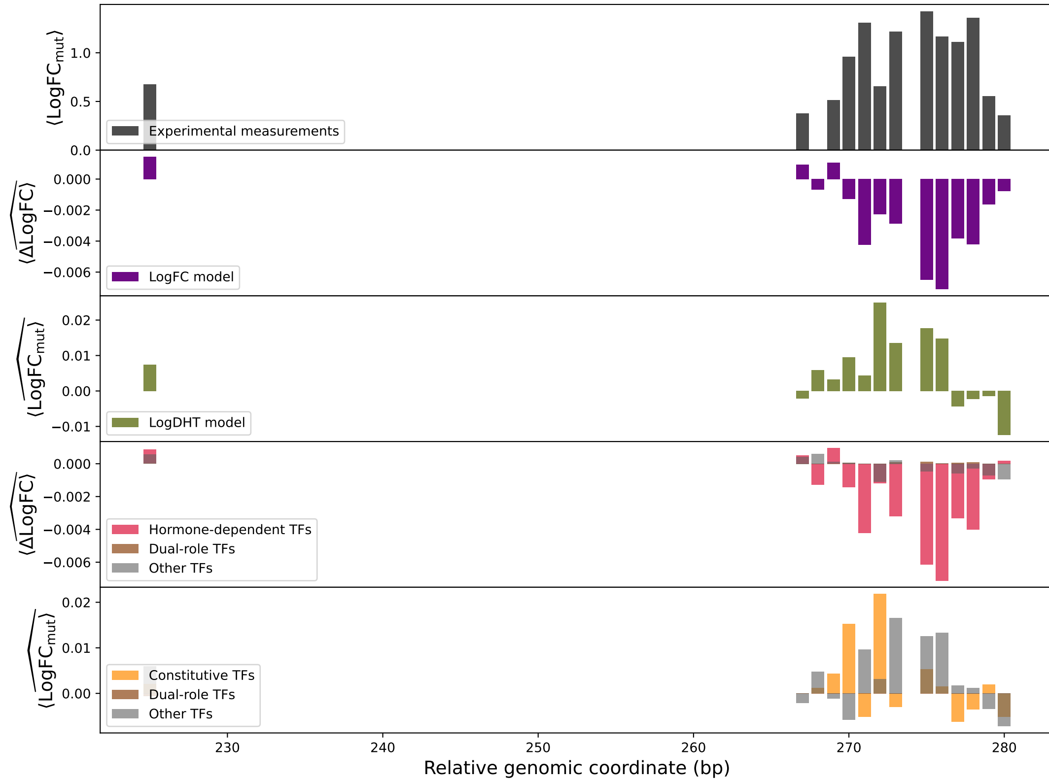
peakno_2221
