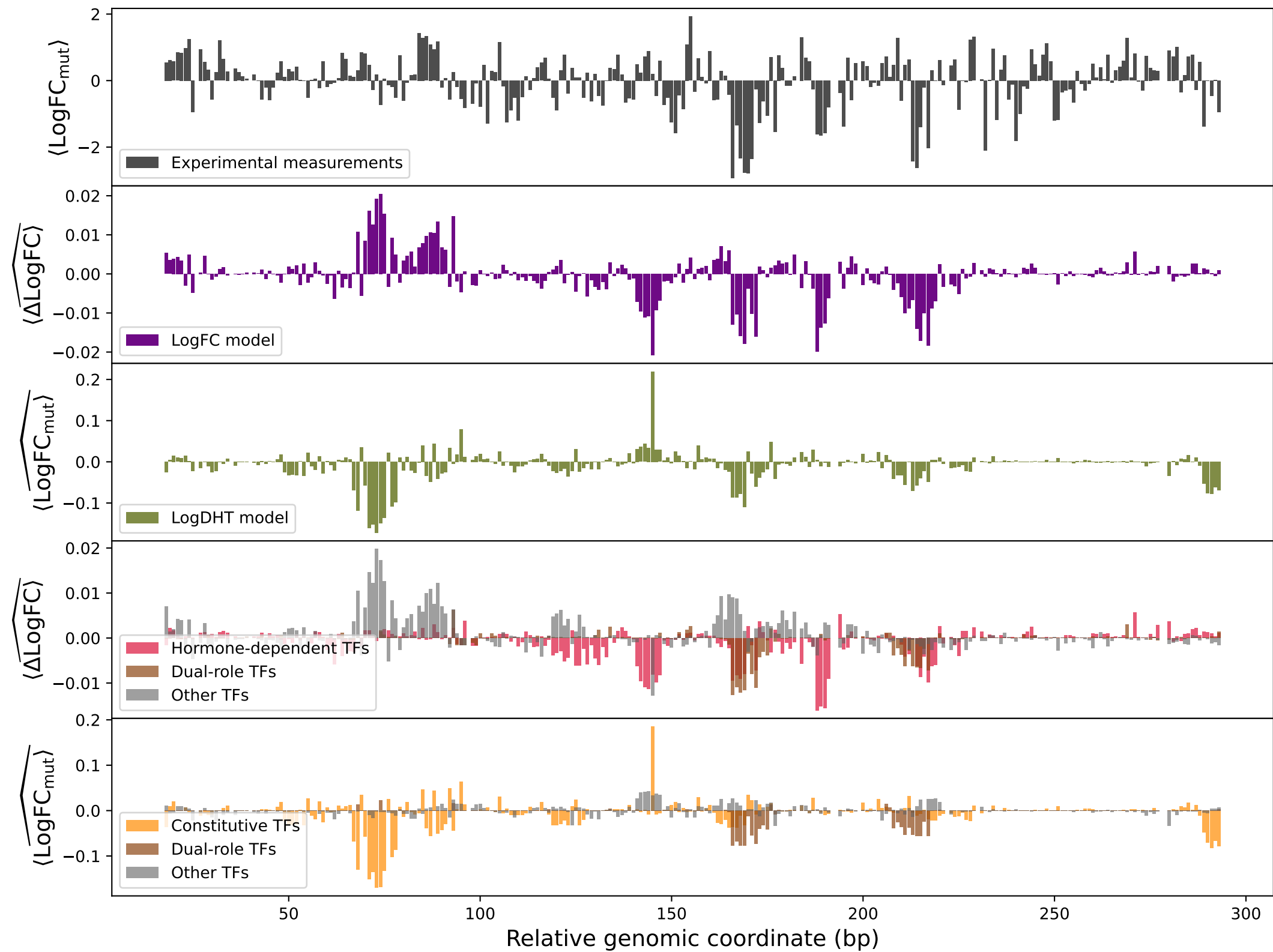
peakno_2261
