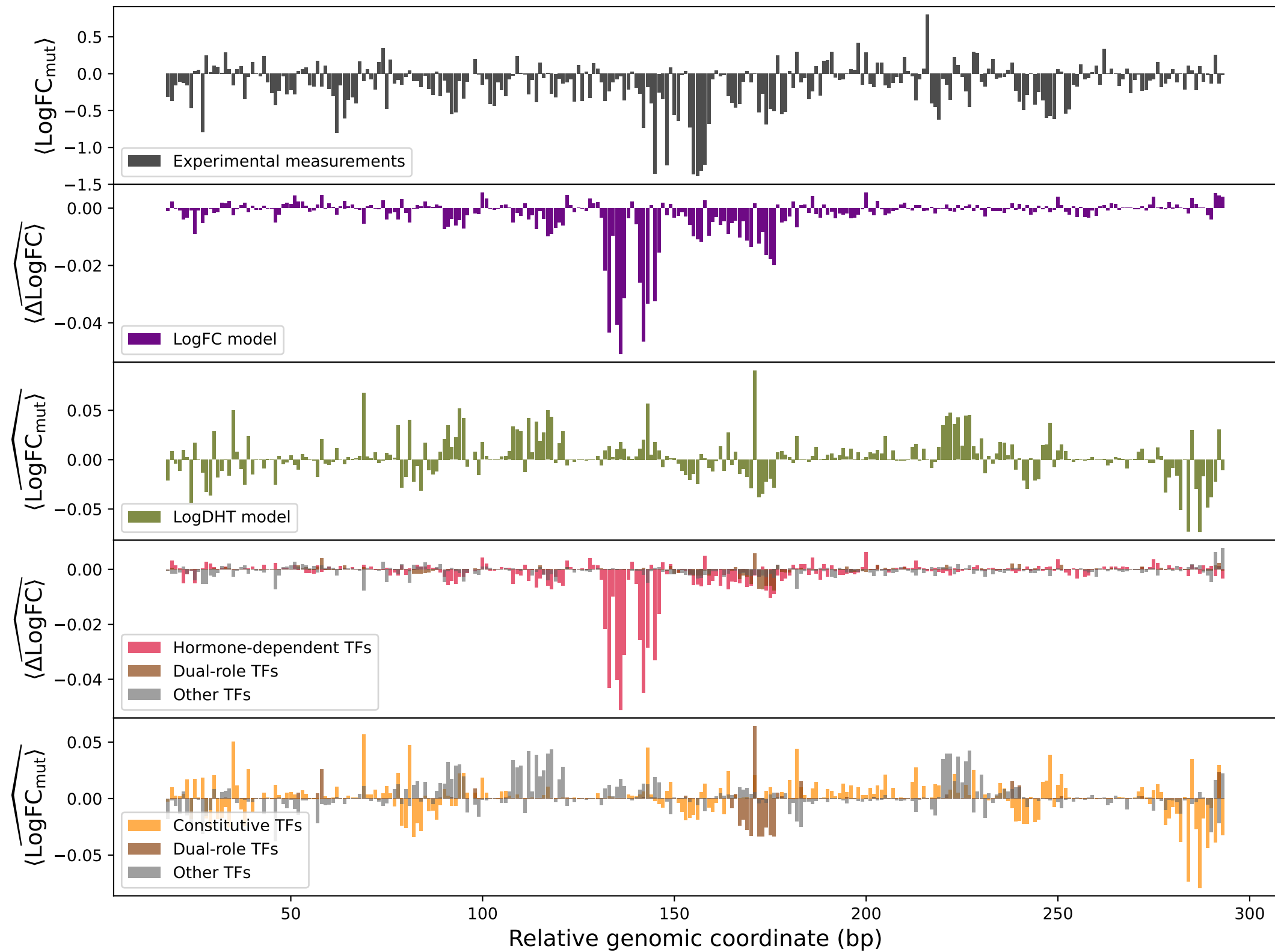
overlapped_read_612
