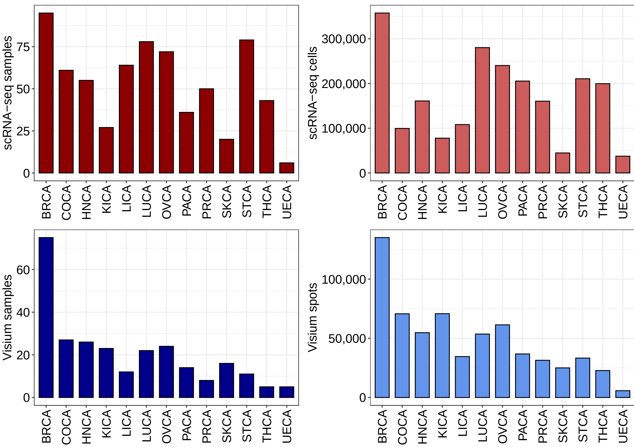
Figure 1a: sample, cell and spot counts by cancer type
