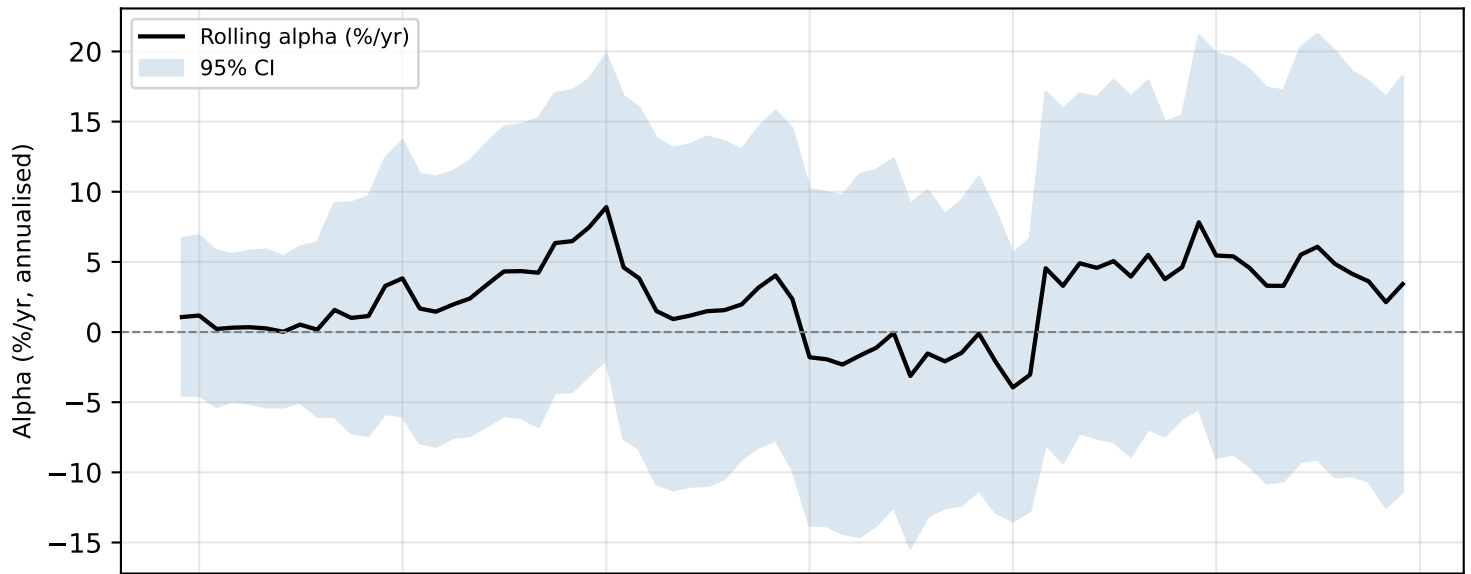
Rolling 36-month FF5+UMD alpha of narrative tercile spread (2016-2024)
