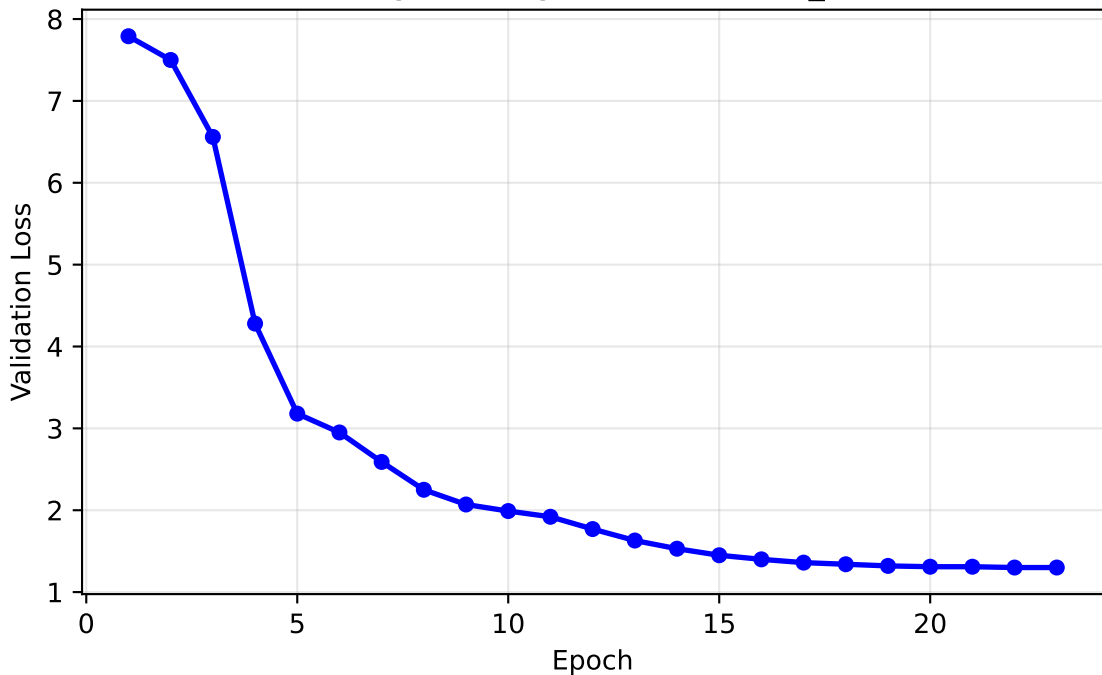
BPT Fine-Tuning Convergence (H20, max_len=10,000)
