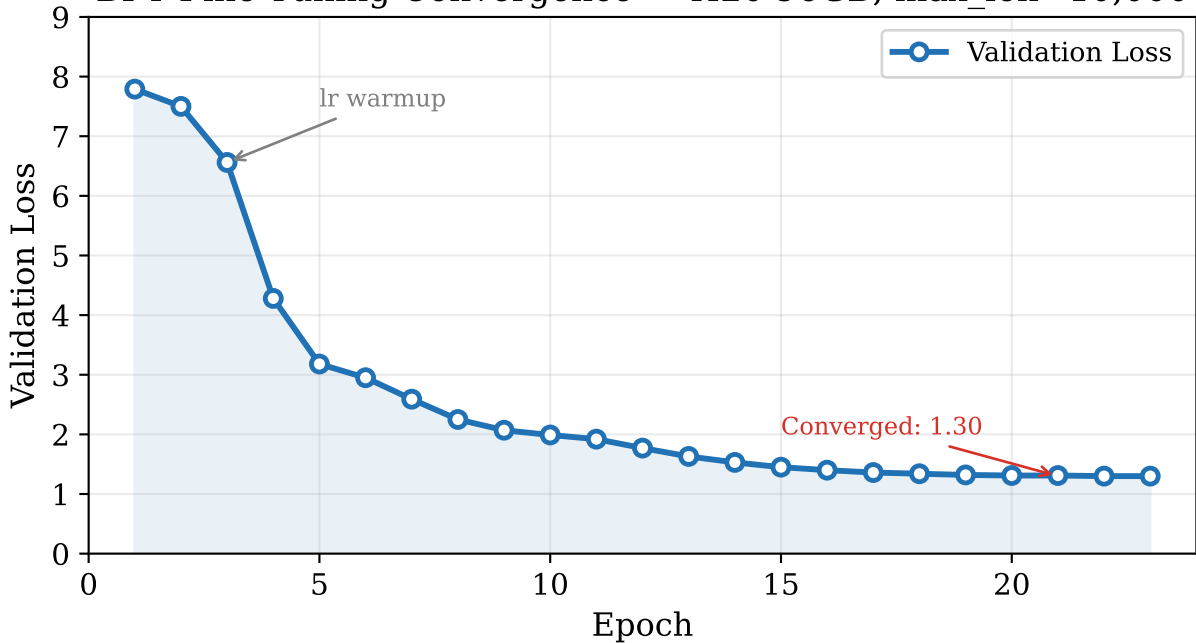
BPT Fine-Tuning Convergence — H2O 96GB, max_len=10,000
