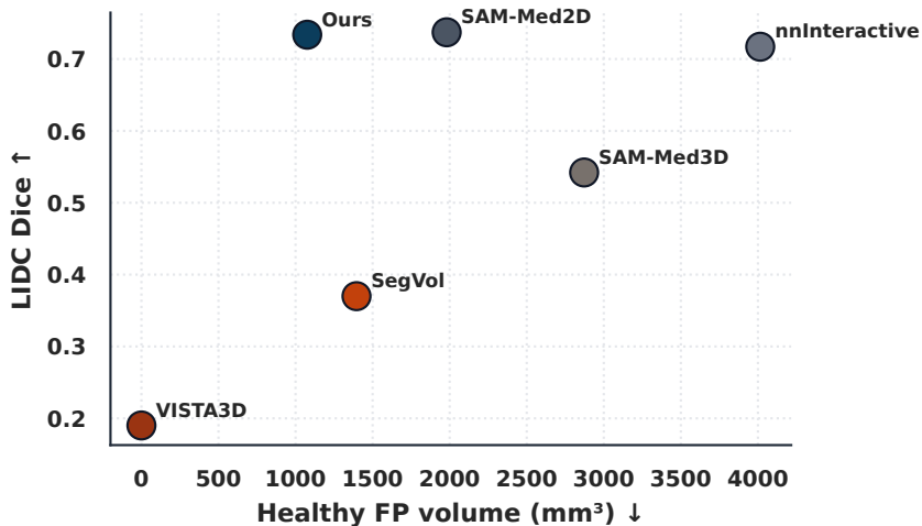
Dice vs FP volume
