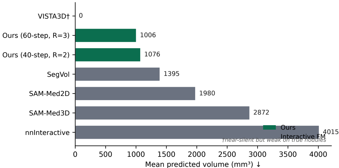
Healthy FP probe: random boxes in nodule-free lung (N=3840)
