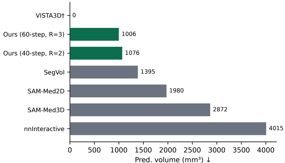
(b) Healthy random-box FP
