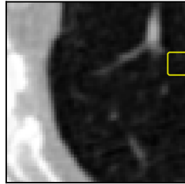
nnInteractive
