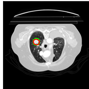
nnInteractive
