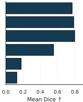
dataset = NSCLC
