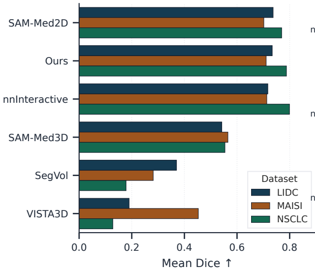
Matched box prompts · all methods
