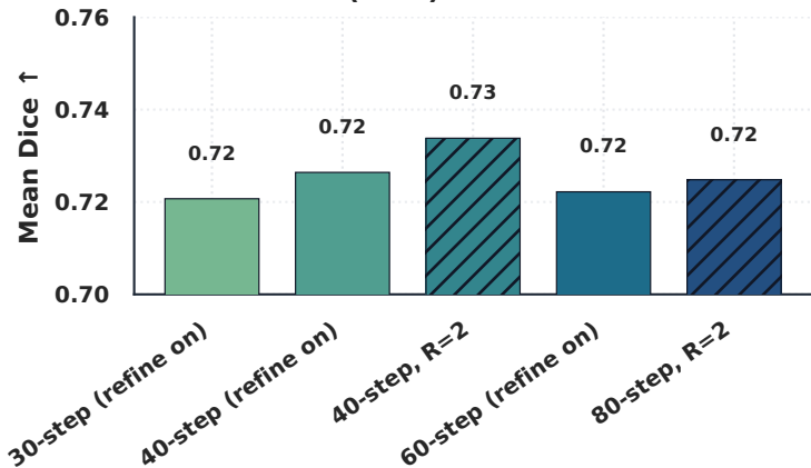
Ours ablation (LIDC)
