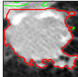
60-step
