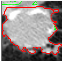
40-step
