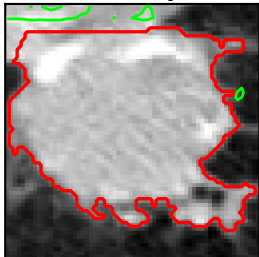
30-step
