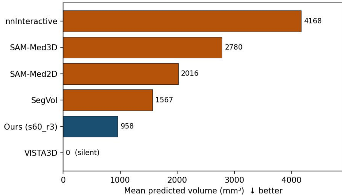
(a) MAISI healthy + random boxes — FP volume
