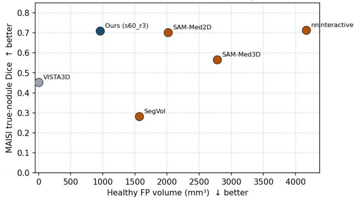
(b) Trade-off: real nodules vs healthy FPs
