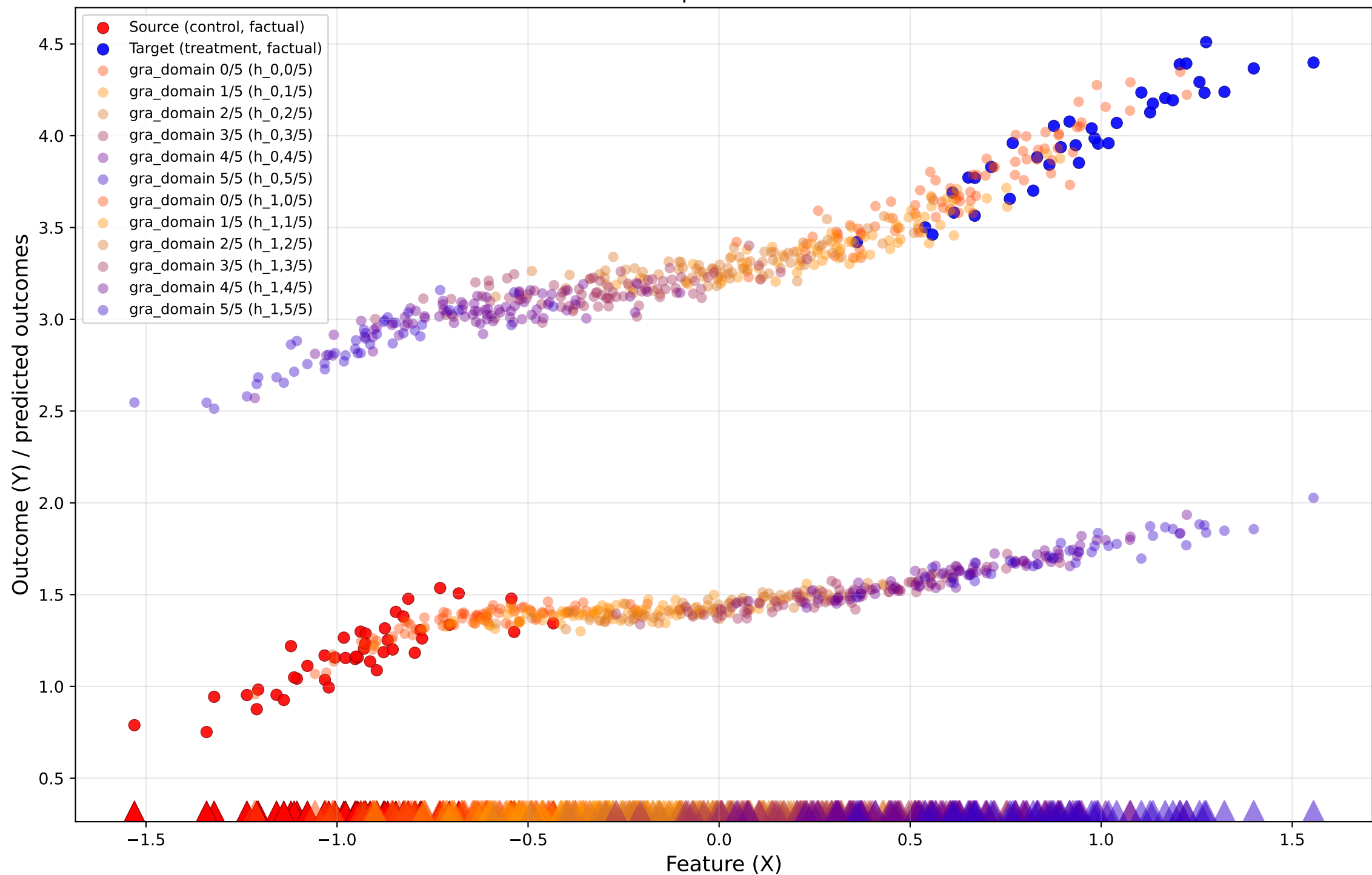
2D Gradual Domain Adaptation with Predicted Outcome
