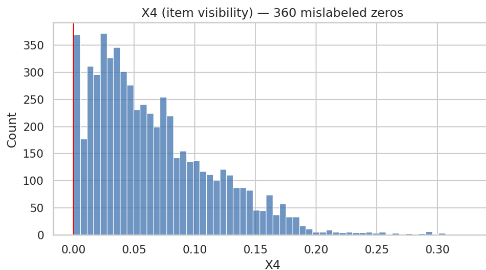
Figure 4: X4 visibility has an abnormal spike at exactly zero, treated as missingness.
