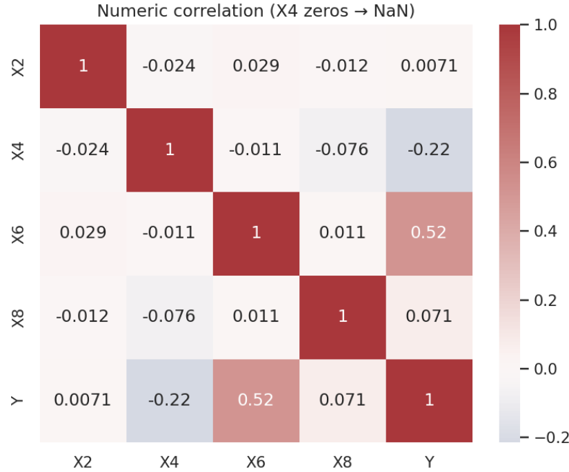
Figure 8: Numeric correlation plot. X6 is the most important raw numeric signal.
