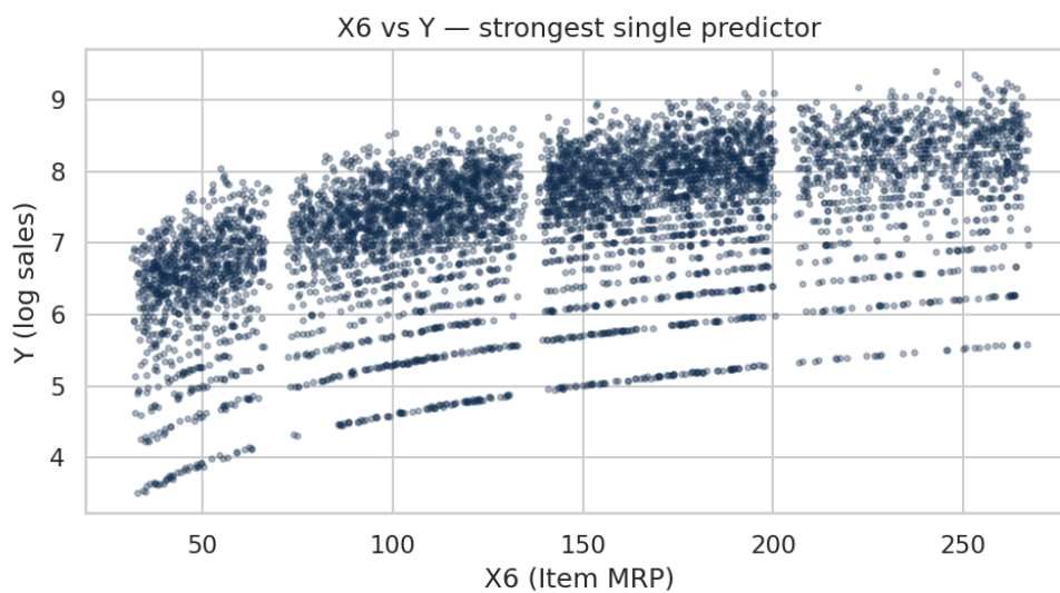
Figure 5: X6 is a strong predictor of the target.
