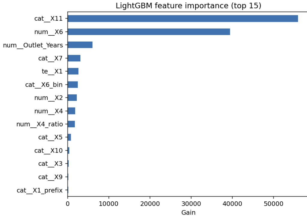
Figure 9: LightGBM feature importance.
