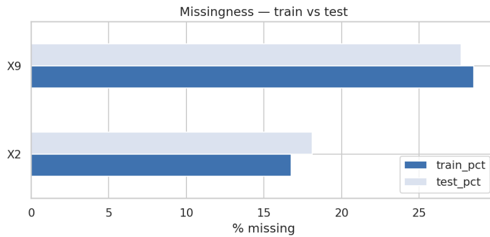
Figure 2: Missingness summary. X2 and X9 are the main columns with missing values.
