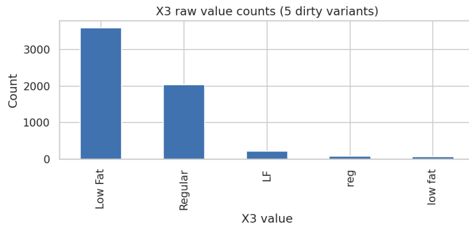
Figure 3: Dirty values in X3. Multiple labels represent the same fat-content classes.
