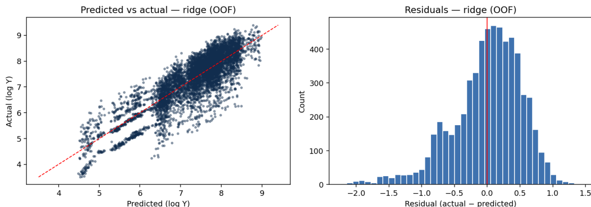
Figure 10: Predicted vs actual and residual histogram.
