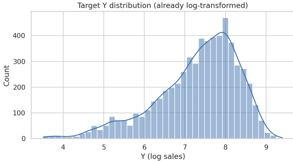
Figure 1: Target distribution. Y is already log-transformed and lies mostly between 3.5 and 9.4.
