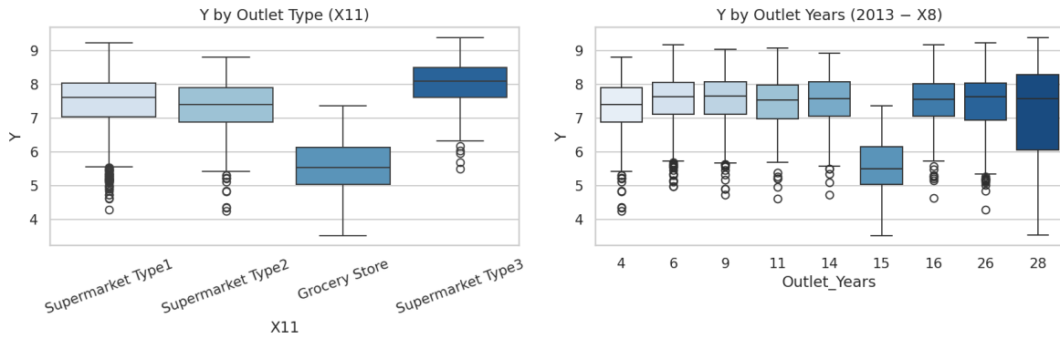
Figure 7: Outlet type and outlet age show systematic target differences.
