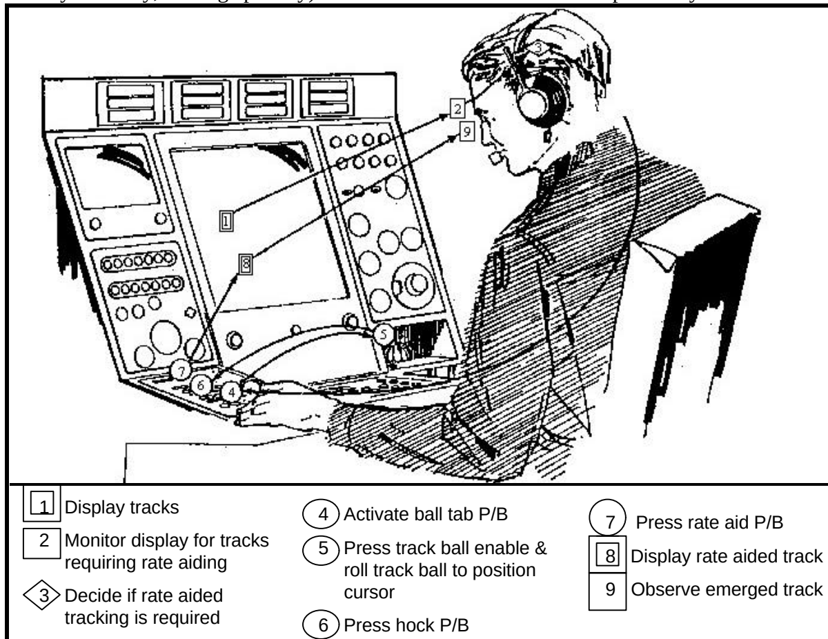
FIGURE 29. Spatial operational sequence diagram (sample) .
