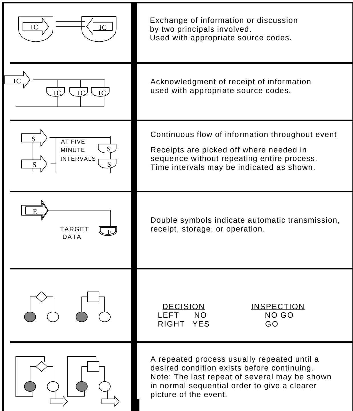
FIGURE 14. Special combinations of OSD symbols.
