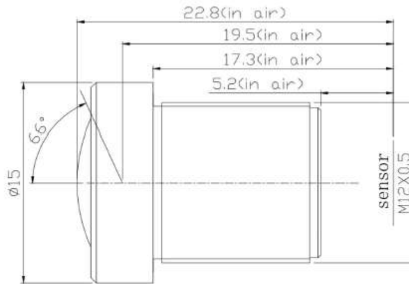
Figure 3: Lens Mechanical Dimensions
