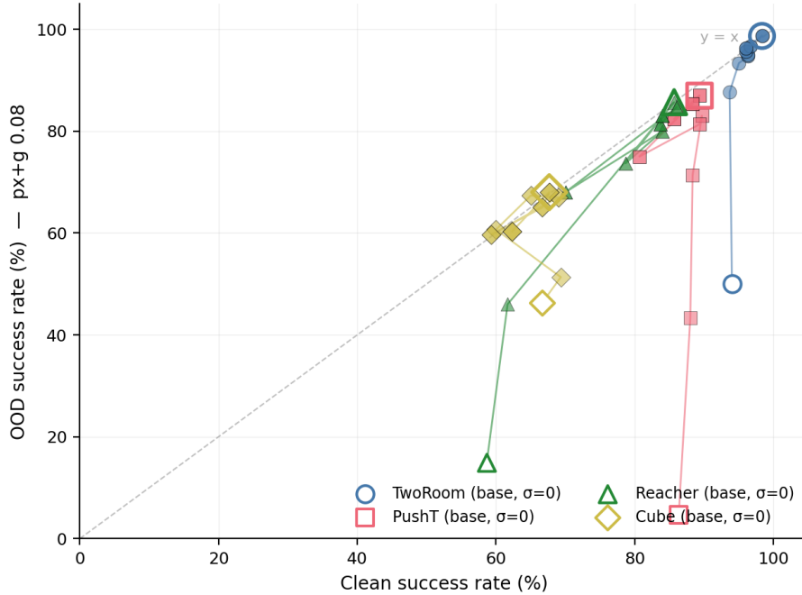
Fig. 6. Per-task Pareto trajectory of (clean, OOD) under noise sweep (open marker = base; solid markers = std_max sweep; ringed marker = px+g 0.08 point-best)
