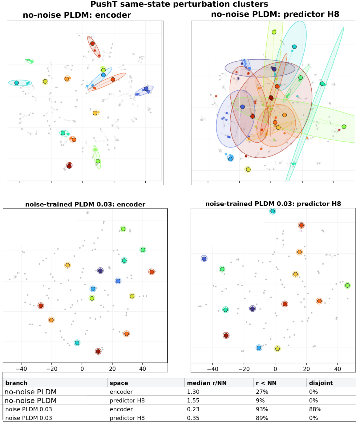
Figure 7: Qualitative PLDM PushT same-state perturbation clusters for Table 21. Top: no-noise-trained PLDM; bottom: noise-trained PLDM at \sigma_{\max} = 0.03 . The embedded table reports original-space local statistics; t-SNE coordinates are qualitative and not comparable with LeWM.
