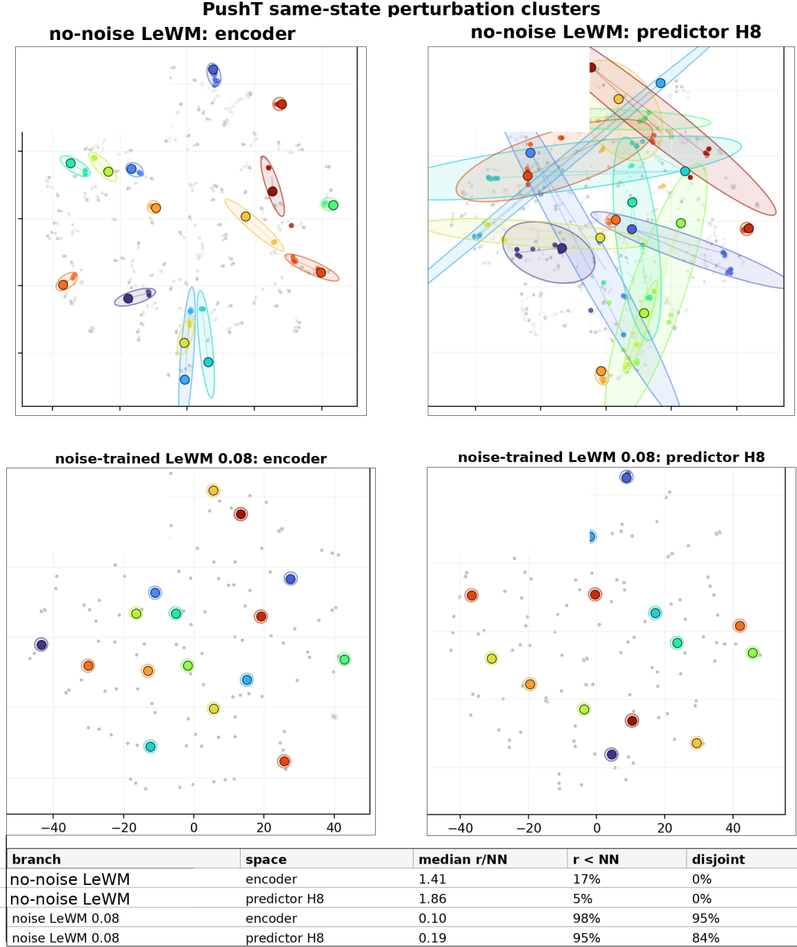
Figure 3: Representative PushT same-state perturbation clusters for Table 4. Top: no-noise-trained LeWM; bottom: noise-trained LeWM at \sigma_{\max} = 0.08 . Left: encoder-history features; right: H = 8 predictor-rollout features. t-SNE coordinates and envelopes are visualization only; the embedded table reports original-space local statistics.
