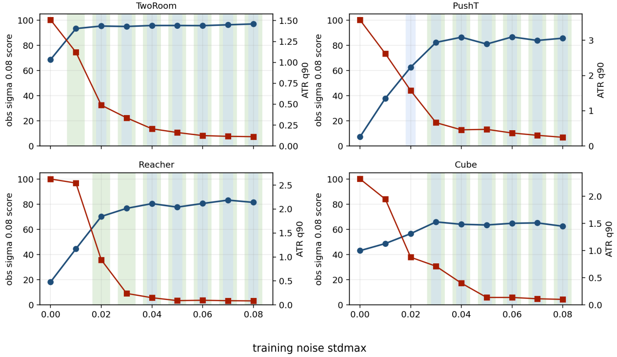
Figure 3: Diagnostic validation of the radius-margin proxy against the Gaussian recovery band. Green bands mark behavioral recovery-band points defined only from closed-loop observation-noise scores; blue bands mark positive fixed-pool proxy gaps computed from fixed-pool diagnostic summaries. ATR is overlaid as the same-state radius-tail side. The shaded diagnostic region is derived from diagnostic statistics only; the behavioral recovery band is shown after the fact for alignment. This is a diagnostic validation, not a new checkpoint-selection algorithm.
