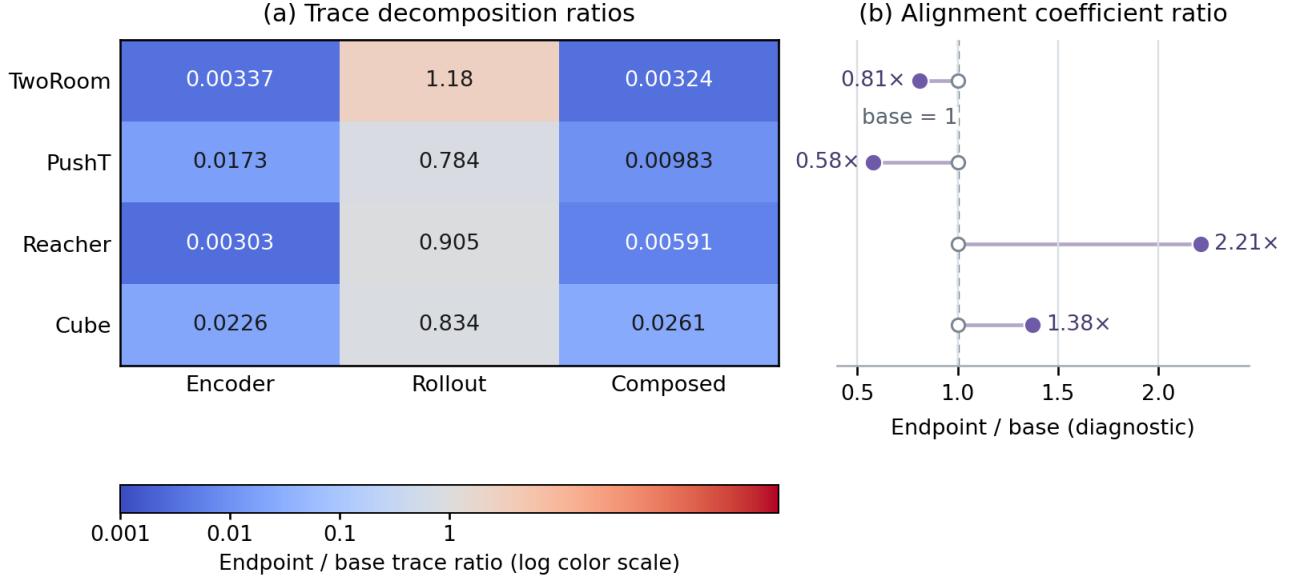
Figure 9: JVP/Hutchinson decomposition behind the local sensitivity audit. Trace ratios show encoder, rollout, and composed endpoint/base sensitivity estimates; the alignment coefficient is displayed separately because it is not the same scale as the trace quantities. These local diagnostics explain where composed sensitivity changes, but they do not provide a global or closed-loop guarantee.
