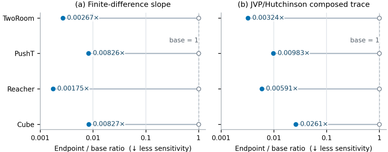
Figure 5: Both local sensitivity estimators drop below their no-noise baselines at the noise-trained endpoint. Finite-difference slopes estimate small-noise rollout-radius response along sampled Gaussian perturbations; exact-autograd JVP/Hutchinson traces estimate local Frobenius averages of the composed encoder-rollout map. Values are endpoint/base ratios within each task; ratios below one support reduced local composed sensitivity, not a global robustness guarantee.
