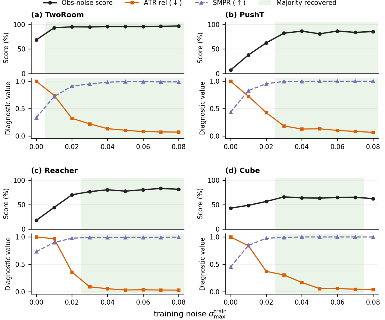
Figure 3: Recovered rows align with lower ATR and stronger margin preservation across the Gaussian training grid. Each task block averages training seeds 3072/3073/3074 at the same \sigma_{\max} value and separates the observation-noise score (upper axis) from normalized ATR tail and direct SMPR at margin zero (lower axes; ATR \downarrow , SMPR \uparrow ). Continuous green bands mark training-noise ranges where a majority of seed rows meet the behavioral recovery criterion. Planner-side top-1 disagreement is separated into Appendix E.
