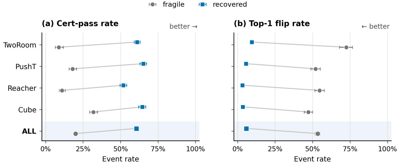
Figure 4: Recovered rows certify more fixed-pool histories and flip fewer top candidates. Cert-pass denotes sampled histories where the maximum paired cost drift over the shared 65-candidate pool is below one half of the clean top-1/top-2 margin; top-1 flip is the observed clean/noisy fixed-pool top-candidate disagreement. Intervals are Wilson 95% intervals over sampled anchors and quantify event-rate uncertainty, not calibrated theorem probabilities. Exact rates, including conditional flip given cert-pass, are in Appendix E.2.
