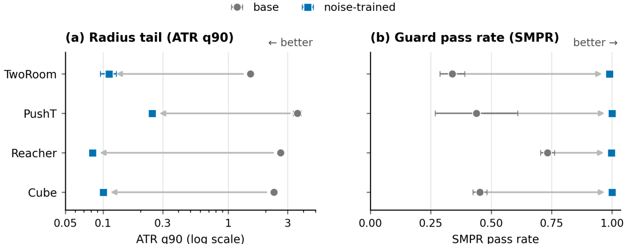
Figure 2: Noise-trained endpoints contract the ATR radius tail and improve the SMPR guard on all four tasks. ATR is the q90 same-state clean/noisy action-conditioned rollout disagreement normalized by the clean transition scale; SMPR is the task-grounded near-boundary selective-margin pass rate. Points report mean across training seeds 3072/3073/3074 and horizontal bars report population standard deviations. Exact values are in Appendix D.
