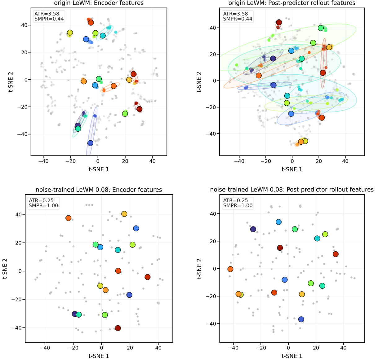
Figure 2: Qualitative PushT ACPC neighborhood t-SNE visualization for the origin LeWM versus \sigma_{\max} = 0.08 noise-trained contrast. The four panels show encoder features and post-predictor rollout features for repeated same-state perturbation views; colored clusters mark fixed random anchors. The t-SNE projection is qualitative. ATR and SMPR are the quantitative diagnostics and are computed in the original projected-rollout diagnostic space.
