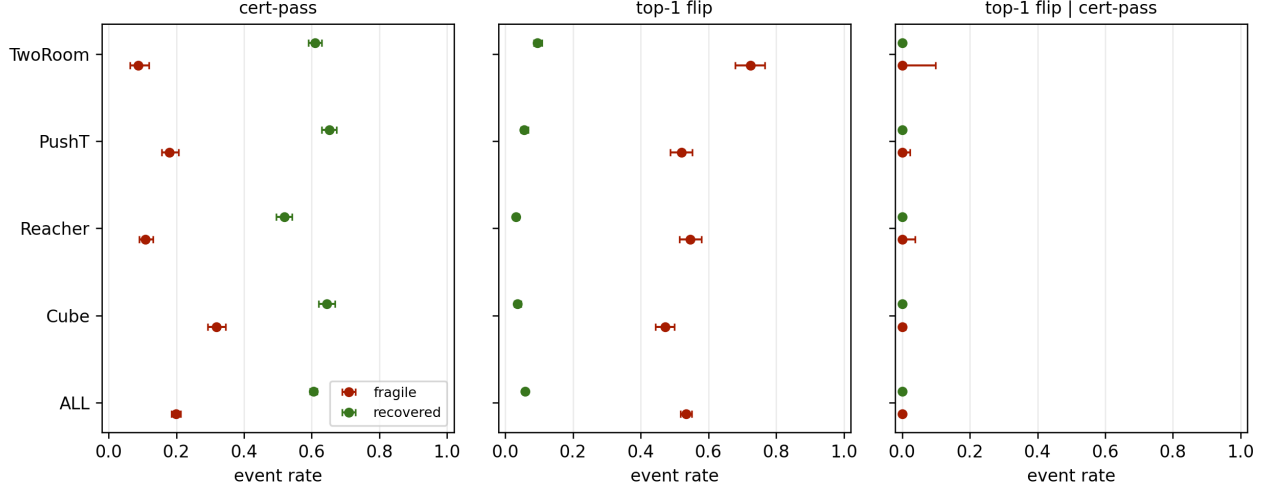
Figure 6: Fixed-pool radius-margin event-rate audit. Cert-pass denotes sampled histories where the maximum paired cost drift over the shared 65-candidate pool is below one half of the clean top-1/top-2 margin. Top-1 flip is the observed clean/noisy fixed-pool top-candidate disagreement. Intervals are Wilson 95% intervals over sampled anchors and quantify event-rate uncertainty, not calibrated theorem probabilities. Exact rates are in Appendix E.2.
