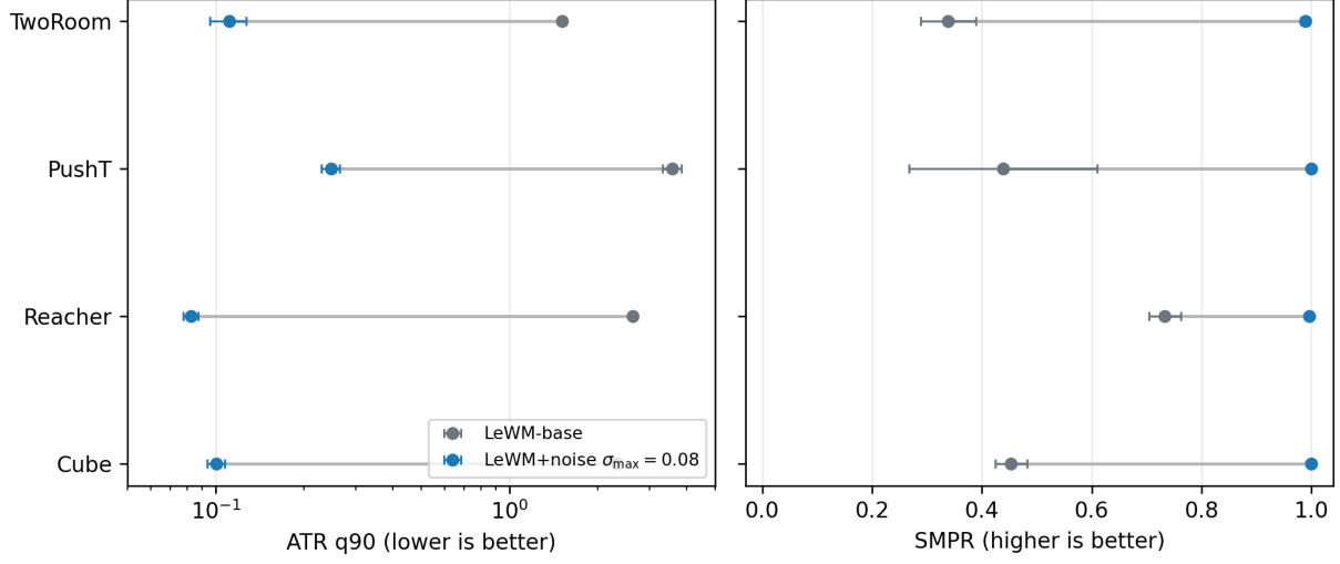
Figure 3: Endpoint selective-ACPC diagnostics over training seeds 3072/3073/3074. ATR is the q90 same-state clean/noisy action-conditioned rollout disagreement; lower is better. SMPR is the task-grounded near-boundary selective-margin pass rate; higher is better. Points report means across training seeds and horizontal bars report population standard deviations. Exact values are in Appendix D.
