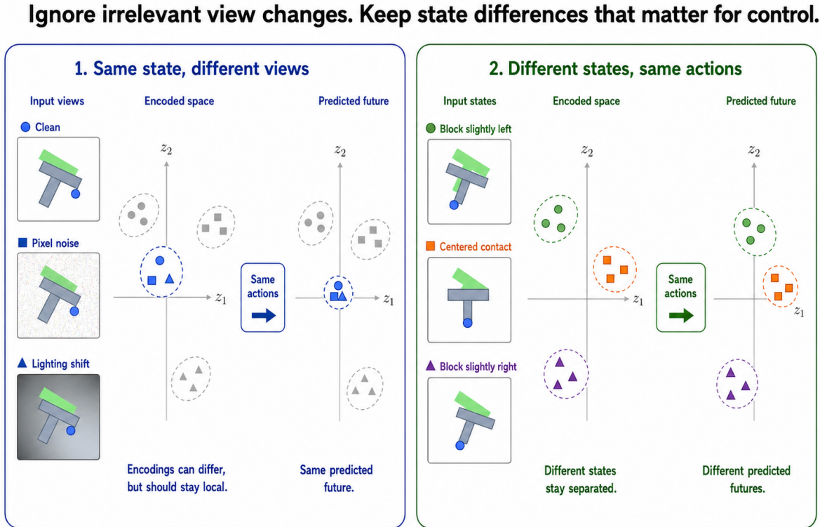
Figure 1: ACPC diagnostic schematic. Clean and perturbed same-state histories are rolled forward under the same action sequence; the radius term measures clean/noisy predictive disagreement, while the guard term requires task- or action-relevant different states to remain separated. The diagnostic is selective: low same-state disagreement is interpreted only together with preserved discriminability.
