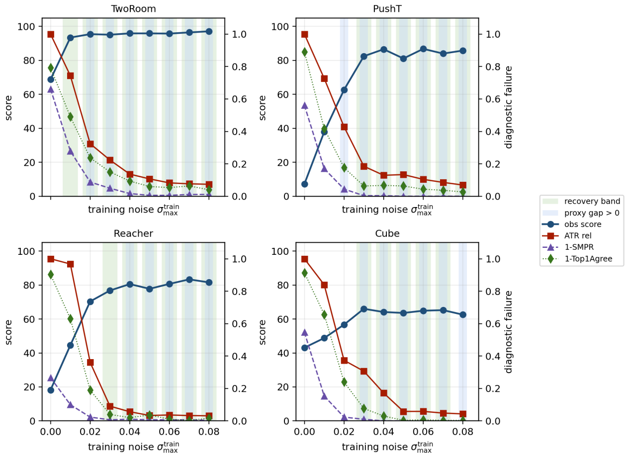
Figure 5: Full-sweep diagnostic separation across the Gaussian training grid. Each task panel averages training seeds 3072/3073/3074 at the same \sigma_{\max} value. Green bands mark behavioral recovery-band points; blue bands mark positive summary-level fixed-pool proxy gaps. The right-axis curves show normalized ATR tail and SMPR failure ( 1 - \text{SMPR} ), plus fixed-pool top-1 disagreement; lower is better for all three diagnostic-failure curves.
