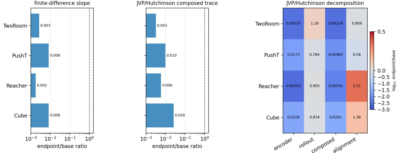
Figure 7: Local Gaussian sensitivity mechanism. Finite-difference slopes estimate small-noise rollout-radius response along sampled Gaussian perturbations; exact-autograd JVP/Hutchinson traces estimate local Frobenius averages of the composed encoder-rollout map. Values are endpoint/base ratios within each task. Ratios below one support reduced local composed sensitivity at the noise-trained endpoint. The decomposition panel reports encoder, rollout, composed, and alignment ratios; these are local mechanism diagnostics rather than global robustness guarantees.
