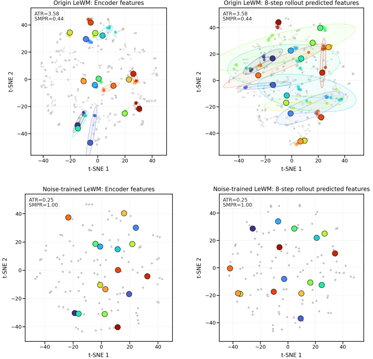
Figure 4: Qualitative PushT ACPC neighborhood t-SNE visualization for the Origin LeWM versus \sigma_{\max} = 0.08 noise-trained contrast. The four panels show encoder features and 8-step rollout predicted features for repeated same-state perturbation views; colored clusters mark fixed random anchors. The t-SNE projection is qualitative. ATR and SMPR are the quantitative diagnostics and are computed in the original projected-rollout diagnostic space.
