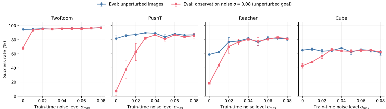
Figure 2: Three-training-seed LeWM Gaussian sweep across four tasks. Each point averages evaluation seeds 42/43/44 within each training seed and then reports mean across training seeds 3072/3073/3074; error bars show population std across training seeds. Blue circles: unperturbed evaluation; red squares: observation-only Gaussian noise \sigma = 0.08 with an unperturbed goal. The curves document broad task-dependent recovery bands rather than checkpoint rankings.
