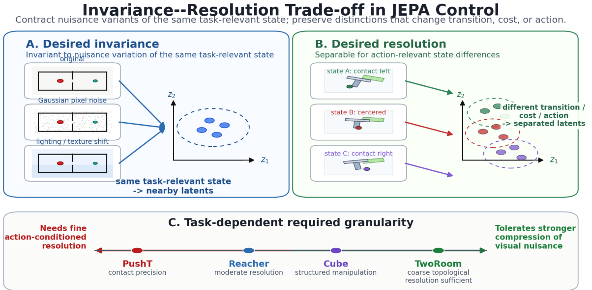
Figure 1: Conceptual reading of the invariance–resolution trade-off. Invariance is beneficial only within equivalence classes of task-relevant state: nuisance variants of the same state should map to nearby latents. States that differ in transition, cost, or optimal action must remain resolvable. The bottom axis is a qualitative task read backed by the sweep and diagnostic evidence; it should not be read as “TwoRoom needs no resolution” or “PushT should preserve all pixels”. PLDM is used as a second-family replication of the task-level signature, while the exact diagnostic mechanism remains method-specific. Section 3 restates this boundary as action-conditioned predictive consistency: contract nuisance perturbations only after the action-conditioned predictor, while keeping action-distinct transitions resolvable.
