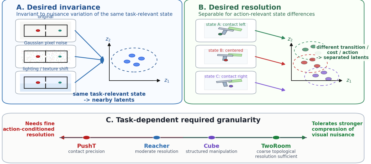
Figure 1: Conceptual reading of the selective-consistency tension. Same-state nuisance variants should induce consistent action-conditioned predictions; states that differ in transition, cost, or optimal action must remain resolvable. The bottom axis is a qualitative task read backed by the sweep and diagnostic evidence; it should not be read as “TwoRoom needs no resolution” or “PushT should preserve all pixels”. PLDM is used as a second-family replication of the task-level signature, while the exact diagnostic mechanism remains method-specific. Section 3 formalises the boundary as action-conditioned predictive consistency: contract nuisance perturbations only after the action-conditioned predictor, while keeping action-distinct transitions resolvable.
