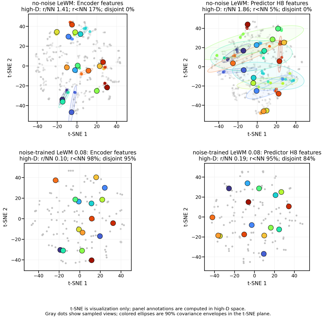
Figure 3: Representative PushT same-state perturbation clusters for Table 3. Top: no-noise-trained LeWM; bottom: noise-trained LeWM at \sigma_{\max} = 0.08 . Left: encoder-history features; right: H = 8 predictor-rollout features. t-SNE coordinates and envelopes are visualization only; the small panel summaries report original-space local statistics.
