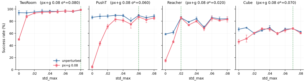
Figure 1: Noise-training sweep: unperturbed vs corrupted evaluation per task. Dashed vertical lines mark each task’s px+g 0.08 point-best \sigma^* . No single std_max is jointly optimal across tasks.
