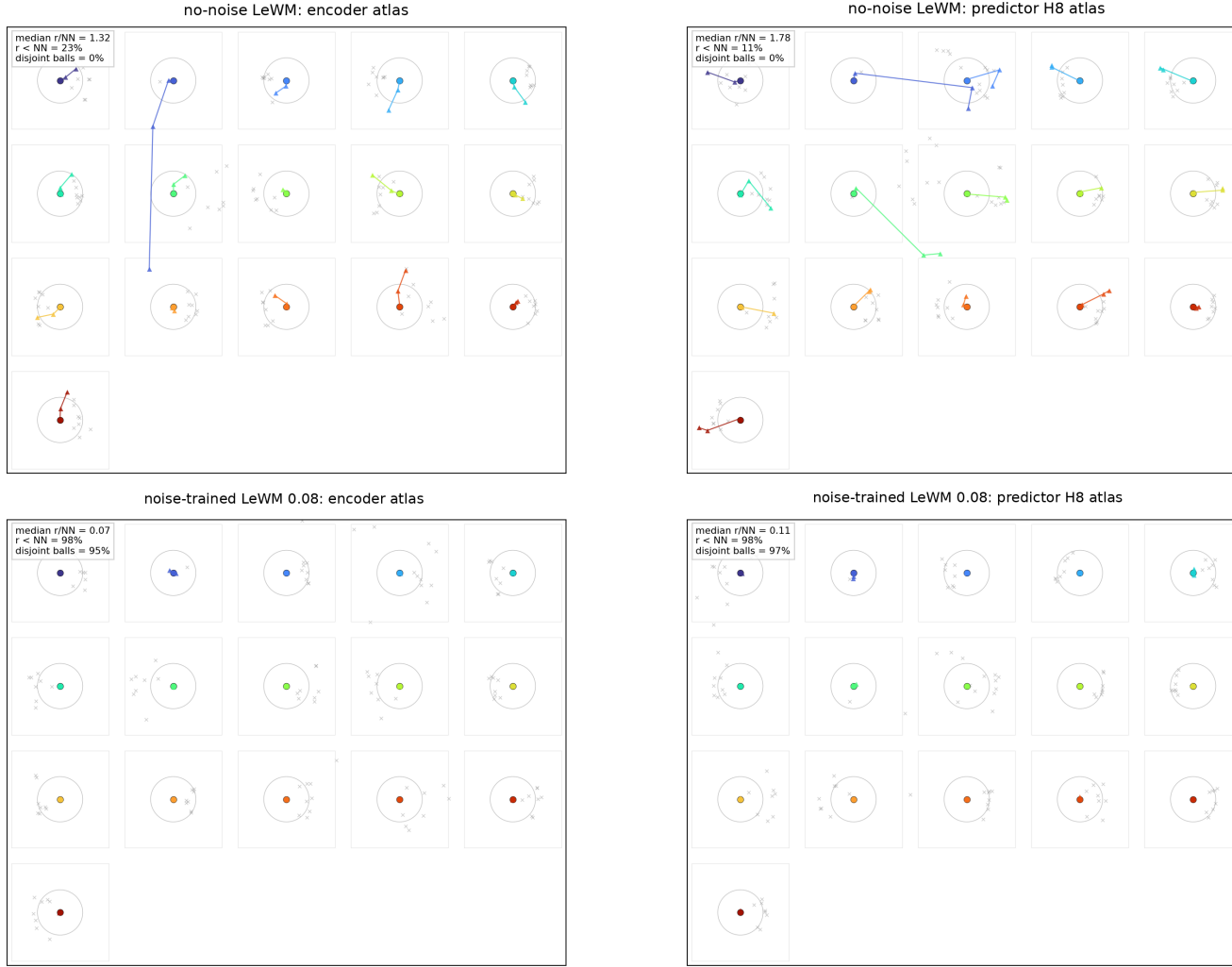
Figure 3: PushT local cluster atlas ( n = 128 windows, 16 anchors, 8 neighbors). Each box is one original state with Gaussian-perturbed views after local PCA; the circle radius is the high-dimensional nearest-other-state distance. Panel summaries report original-space local statistics.
