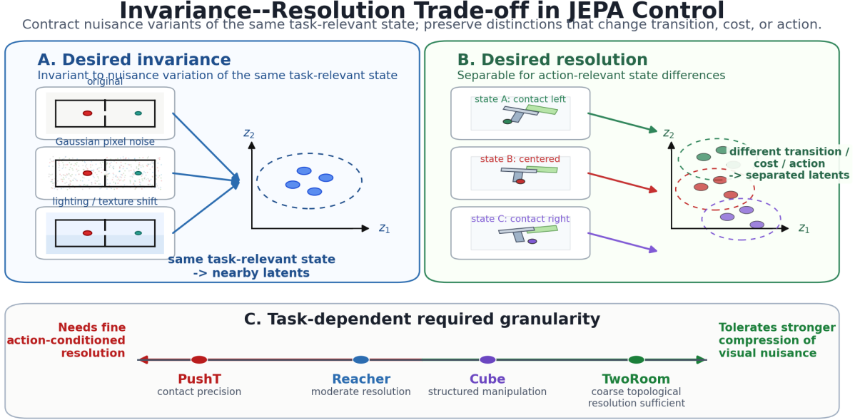
Figure 1: Conceptual reading of the selective-consistency tension. Same-state nuisance variants should induce consistent action-conditioned predictions; states that differ in transition, cost, or optimal action must remain resolvable. The bottom axis is a qualitative task read backed by the sweep and diagnostic evidence; it should not be read as “TwoRoom needs no resolution” or “PushT should preserve all pixels”. PLDM is used as a second-family replication of the task-level signature, while the exact diagnostic mechanism remains method-specific. Section 3 formalises the boundary as action-conditioned predictive consistency: contract nuisance perturbations only after the action-conditioned predictor, while keeping action-distinct transitions resolvable.
