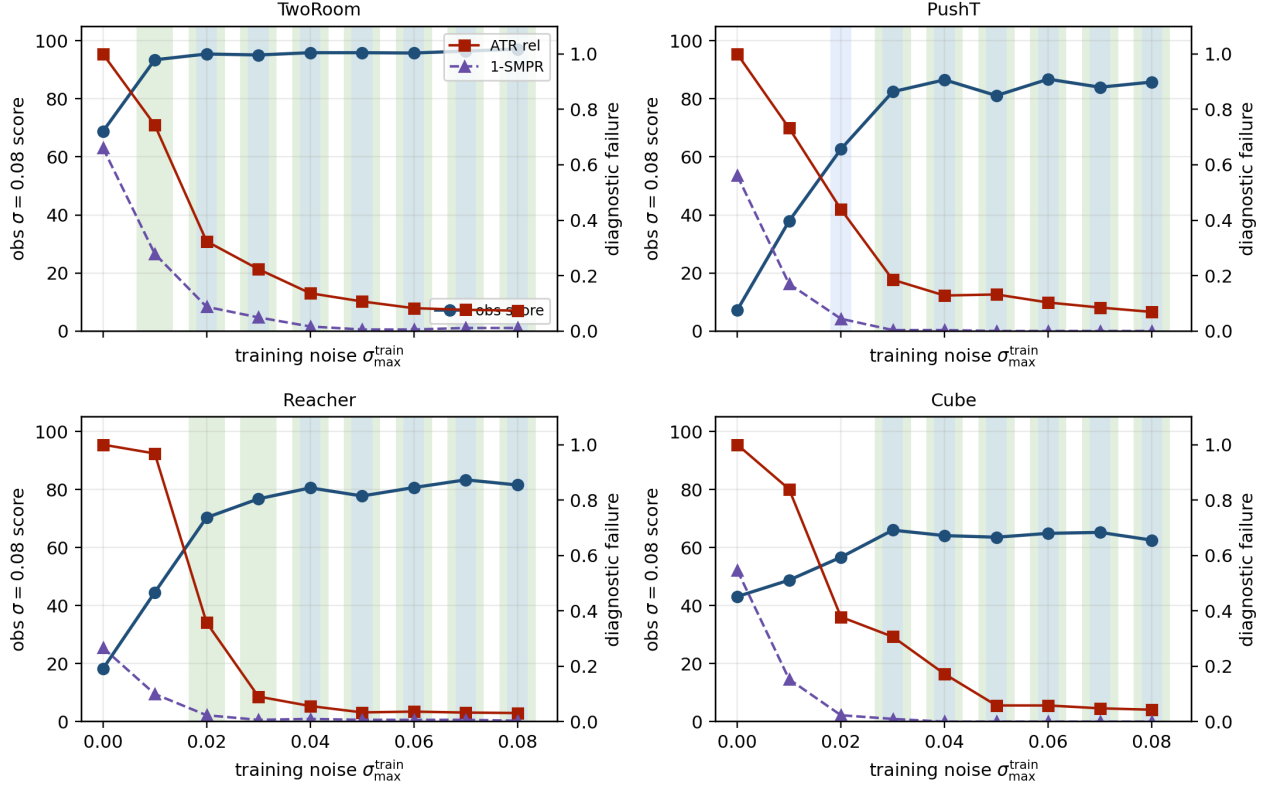
Figure 3: Diagnostic validation of the radius-margin proxy against the Gaussian recovery band. Green bands mark behavioral recovery-band points defined only from closed-loop observation-noise scores; blue bands mark positive fixed-pool proxy gaps computed from retained fixed-pool summaries. The right-axis curves show normalized ATR tail and SMPR failure ( 1 - \text{SMPR} ), both lower-is-better, from the full-sweep diagnostic rows. The shaded diagnostic region is derived from diagnostic statistics only; the behavioral recovery band is shown after the fact for alignment. This is a diagnostic validation, not a new checkpoint-selection algorithm.
