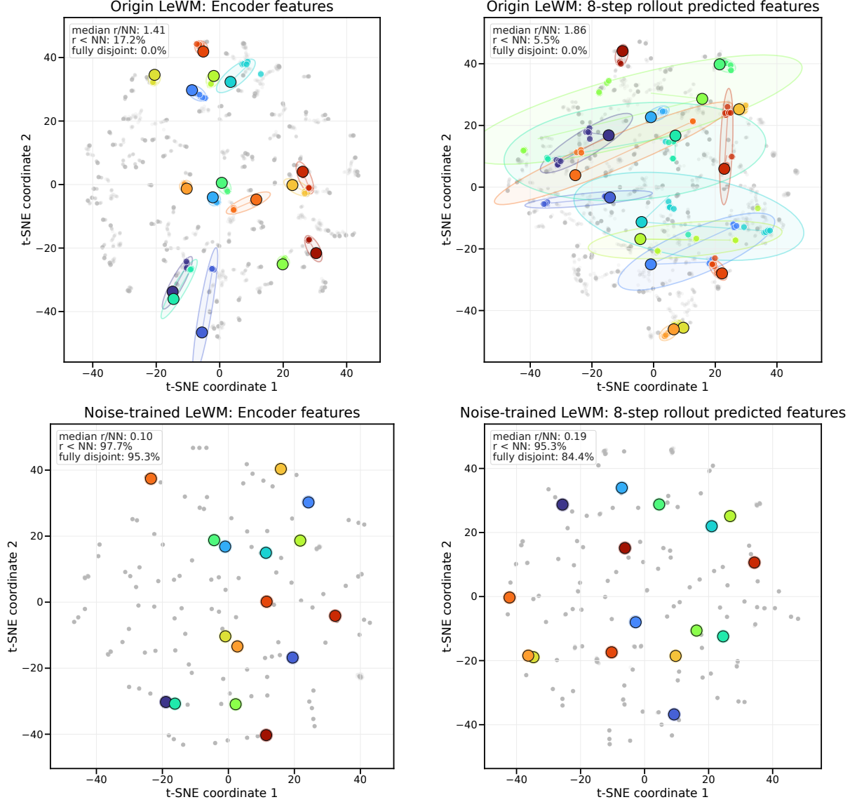
Figure 1: Descriptive local-geometry case study motivating the controlled ACPC comparison. Rows compare a matched pair of PushT checkpoints: one unaugmented and one trained with Gaussian augmentation at \sigma_{\max} = 0.08 ; columns show the encoder output and the representation after eight autoregressive rollout steps. Each color denotes one of 16 highlighted histories: the large black-rimmed marker is its clean anchor, smaller same-color markers are its 18 perturbed views, and the faint ellipse is their 90% t-SNE envelope; gray points show all other histories and views. Under strong contraction, smaller markers and ellipses can lie beneath the clean marker. Each panel’s upper-left summary reports, across all 128 anchors, the median r/NN and the percentages with r < NN and with fully disjoint high-dimensional enclosing balls. The t-SNE coordinates and ellipses are qualitative and enter none of these metrics.
