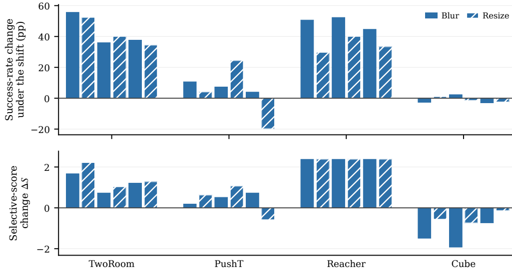
Figure 5: Correspondence between planning gains and the diagnostic under blur and resize for all 24 checkpoint pairs (unaugmented versus \sigma_{\max} = 0.08 ), grouped by task and ordered by training run. Top: success-rate change under the shift. Bottom: selective-score change \Delta S of the same pairs under the common thresholds; hatched bars are resize. Tasks with clear planning gains (TwoRoom, Reacher) also show clearly positive score changes, while Cube changes little in planning and its score decreases.
