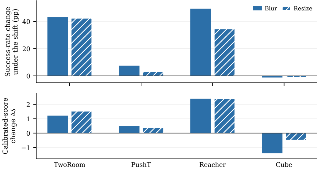
Figure 6: Correspondence between planning gains and the diagnostic under blur and resize. Bars average the three training runs for each task and shift; per-pair values are in Table 10. Top: change in planning success rate from the unaugmented to the \sigma_{\max} = 0.08 checkpoint under the shift. Bottom: change \Delta S in the calibrated score of Equation (17), i.e., how much more margin the noise-trained checkpoint has inside the common thresholds; positive means the diagnostic favors it. Tasks with clear planning gains (TwoRoom, Reacher) also gain score; Cube gains neither.
