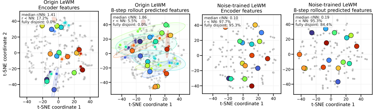
Figure 1: Descriptive local-geometry case study motivating the controlled ACPD comparison. Panels compare a matched pair of PushT checkpoints—the left two unaugmented, the right two trained with Gaussian augmentation at \sigma_{\max} = 0.08 —at the encoder output and after eight autoregressive rollout steps. Each color denotes one of 16 highlighted histories: the large black-rimmed marker is its clean anchor, smaller same-color markers are its 18 perturbed views, and the faint ellipse is their 90% t-SNE envelope; gray points show all other histories and views. Under strong contraction, smaller markers and ellipses can lie beneath the clean marker. Each panel’s upper-left summary reports, across all 128 anchors, the median r/NN and the percentages with r < NN and with fully disjoint high-dimensional enclosing balls. The t-SNE coordinates and ellipses are qualitative and enter none of these metrics.
