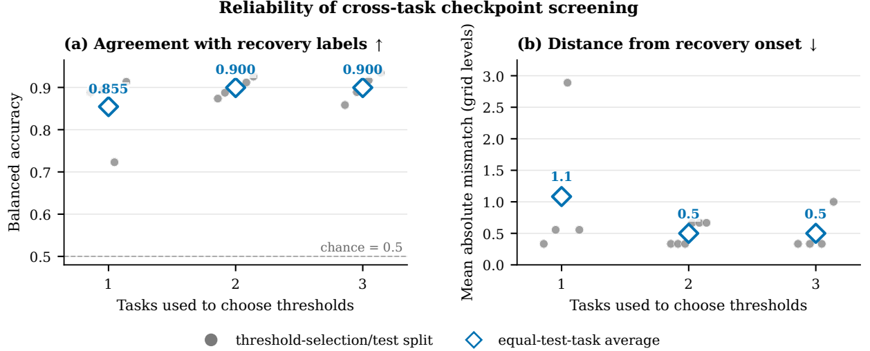
Figure 5: Reliability of checkpoint screening when ATR–SMPR thresholds are chosen on other tasks. A checkpoint passes when relative ATR \leq t_R and SMPR \geq t_M . (a) Agreement with recovery labels on test tasks, measured by balanced accuracy (chance is 0.5). (b) Distance between the diagnostic and behavioral recovery onsets, measured in training-augmentation grid levels (one level is 0.01 in \sigma_{\max} ). Gray points are individual threshold-selection/test partitions; diamonds average test tasks equally for each number of threshold-selection tasks.
